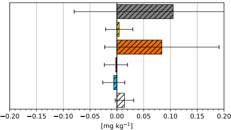
(g) - Total water (H 2 O + IWC)
