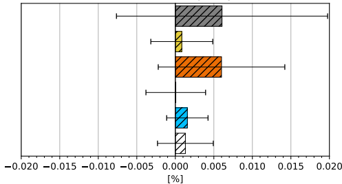
(h) - Cloud frequency
