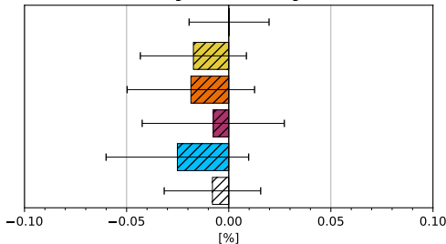
(g) - Total water (H 2 O + IWC)
