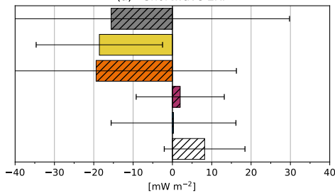
(c) - Shortwave ERF (clear-sky)
