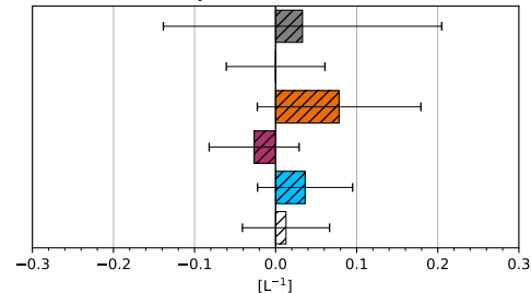
(h) - Cloud frequency
