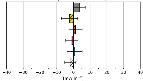
(f) - Ice crystal number concentration
