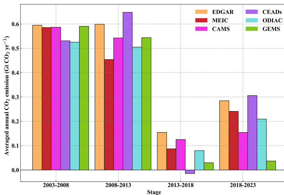
Figure 2. Average annual CO 2 emission growth rate during the 5-year periods.
