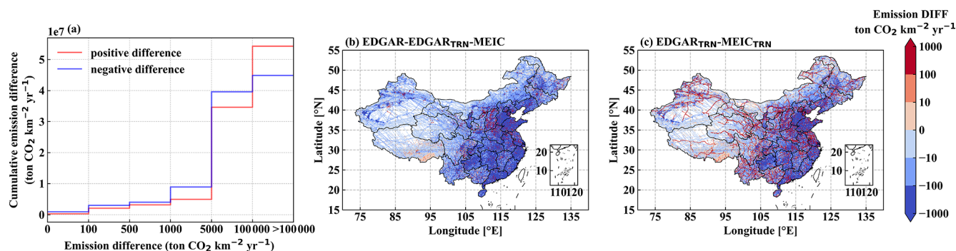
Figure 6. (a) Cumulative distribution of gridded emission differences ( \text{t CO}_2 \text{ km}^{-2} \text{ yr}^{-1} ) between EDGAR and MEIC inventories. The cumulative sum for negative differences (blue line) is calculated using their absolute magnitudes and plotted against the corresponding positive values on the x-axis (i.e., 100 represents -100 ). The spatial distributions of the differences are shown in (b) EDGAR emissions without transport minus MEIC total emissions and (c) EDGAR transport emissions minus MEIC transport emissions.
