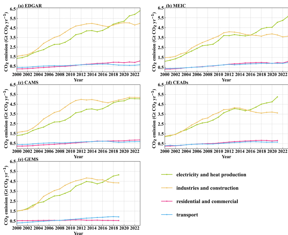
Figure 3. Anthropogenic CO 2 emissions by sector – electricity and heat production, industries and construction, residential and commercial, and transport – for the period 2000–2023, as reported by EDGAR (a), MEIC (b), CAMS (c), CEADs (d), and GEMS (e). Although CEADs provides both national- and provincial-level sectoral data, the national-level version is used here for consistency with other inventories. ODIAC does not provide sectoral CO 2 emissions.
