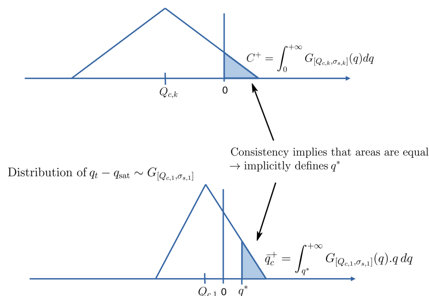
Figure A1. Illustration of integration steps to compute the mean cloud fraction C^+ and the mean condensate content \bar{q}_c^+ within the grid-box with triangular distributions. The first step is the integration of q_t - kq_{\text{sat}} distribution on its positive support in order to compute cloudiness C^+ . The second step is the integration of local cloud contents defined by the q_t - q_{\text{sat}} distribution on the grid-box cloudy part, leading to \bar{q}_c^+ . In this second step, the integration domain is [q^*, +\infty[ where q^* is defined to ensure consistency on cloudiness computation.
