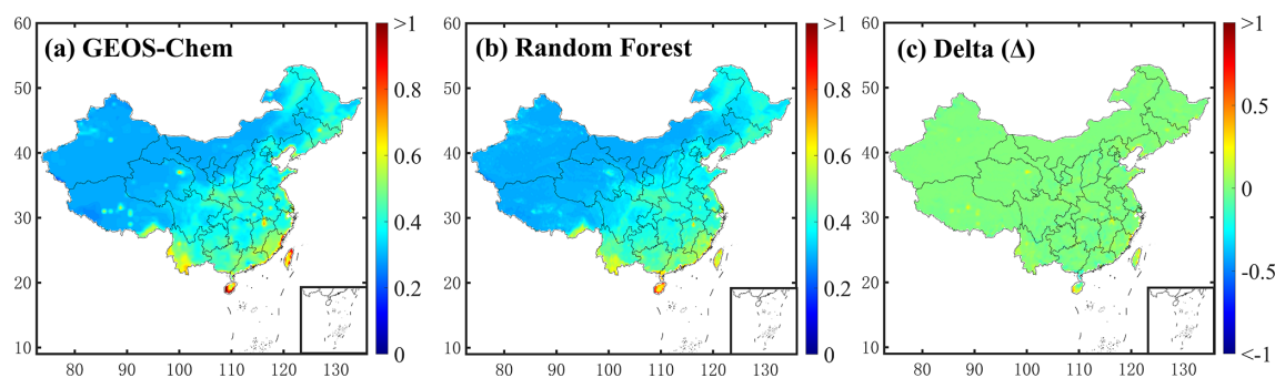
Figure 5. \text{NH}_3 dry deposition velocity in China in 2015: (a) GEOS-Chem simulation; (b) random forest simulation (includes both validation set and training set); (c) model difference (Unit: \text{cm s}^{-1} ).
