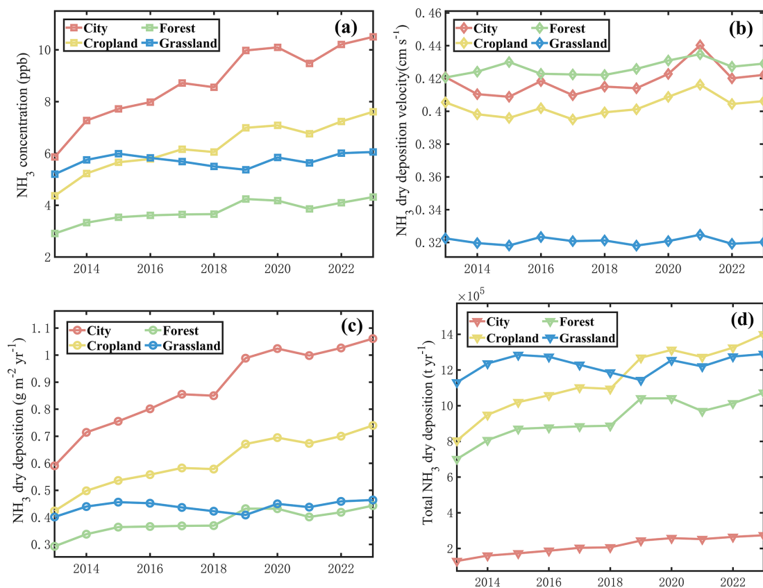
Figure 7. Trends in \text{NH}_3 concentration, dry deposition velocity, and dry deposition amount in China from 2013 to 2023: (a) trends in corrected \text{NH}_3 concentrations across different land surface types (Unit: ppb); (b) \text{NH}_3 dry deposition velocities over different land surface types (Unit: \text{cm s}^{-1} ); (c) trends in \text{NH}_3 dry deposition flux per unit area over different land surface types (Unit: \text{g m}^{-2} ); (d) interannual variation in annual \text{NH}_3 dry deposition over different land cover types (Unit: \text{t yr}^{-1} ).
