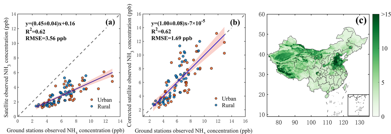
Figure 4. (a) Comparison between CrIS satellite-based column average (from ground to \sim 1 km) \text{NH}_3 concentration and ground site based ( \sim 1.5 m) \text{NH}_3 observations before adjustment; (b) comparison between CrIS satellite-based column average \text{NH}_3 concentration and ground site based \text{NH}_3 observations after adjustment to ground-level; (c) spatial distribution of adjusted satellite-based \text{NH}_3 concentration and comparisons with ground site based \text{NH}_3 concentrations in 2015 (Unit: ppb), note the adjustment from CrIS satellite-based column average (ground to \sim 1 km) to ground-level ( \sim 1.5 m) is conducted by using the linear regression equation derived from panel (a), each scatter plot represents monthly averages of all available observations for either urban or rural site.
