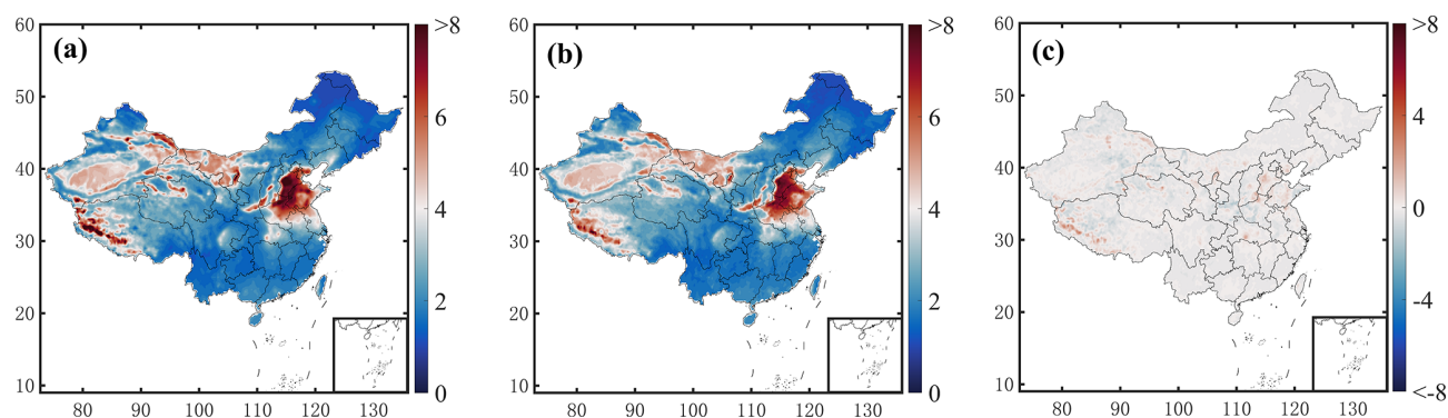
Figure 9. (a) Spatial distribution of adjusted ground-level \text{NH}_3 concentration for averages between 2013 and 2023, (b) simulation of adjusted ground-level \text{NH}_3 concentration by RF model for averages between 2013 and 2023, (c) difference between panel (a) and (b), Units: ppb.
