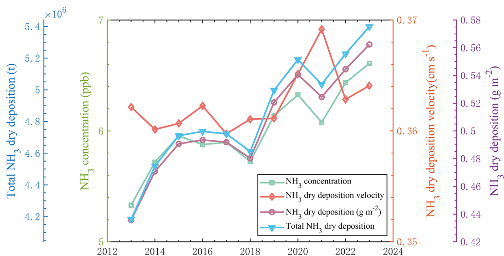
Figure 8. Annual changes in \text{NH}_3 concentration, dry deposition velocity, dry deposition flux and total dry deposition for China from 2013 to 2023.
