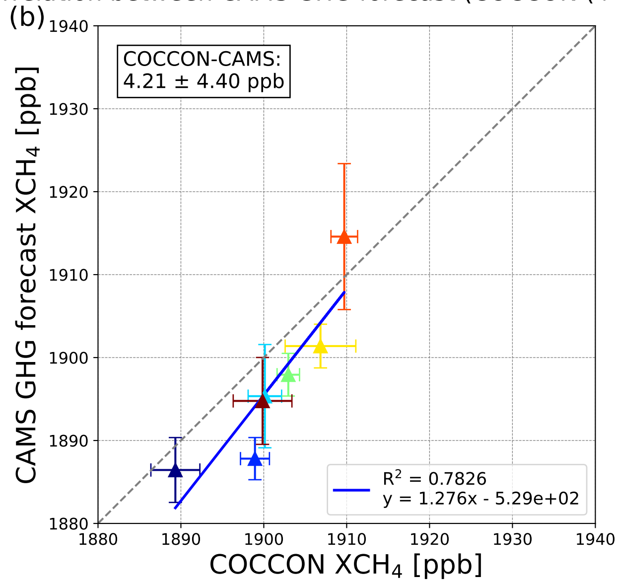
Correlation between CAMS GHG forecast (COCCON (+-2h))
