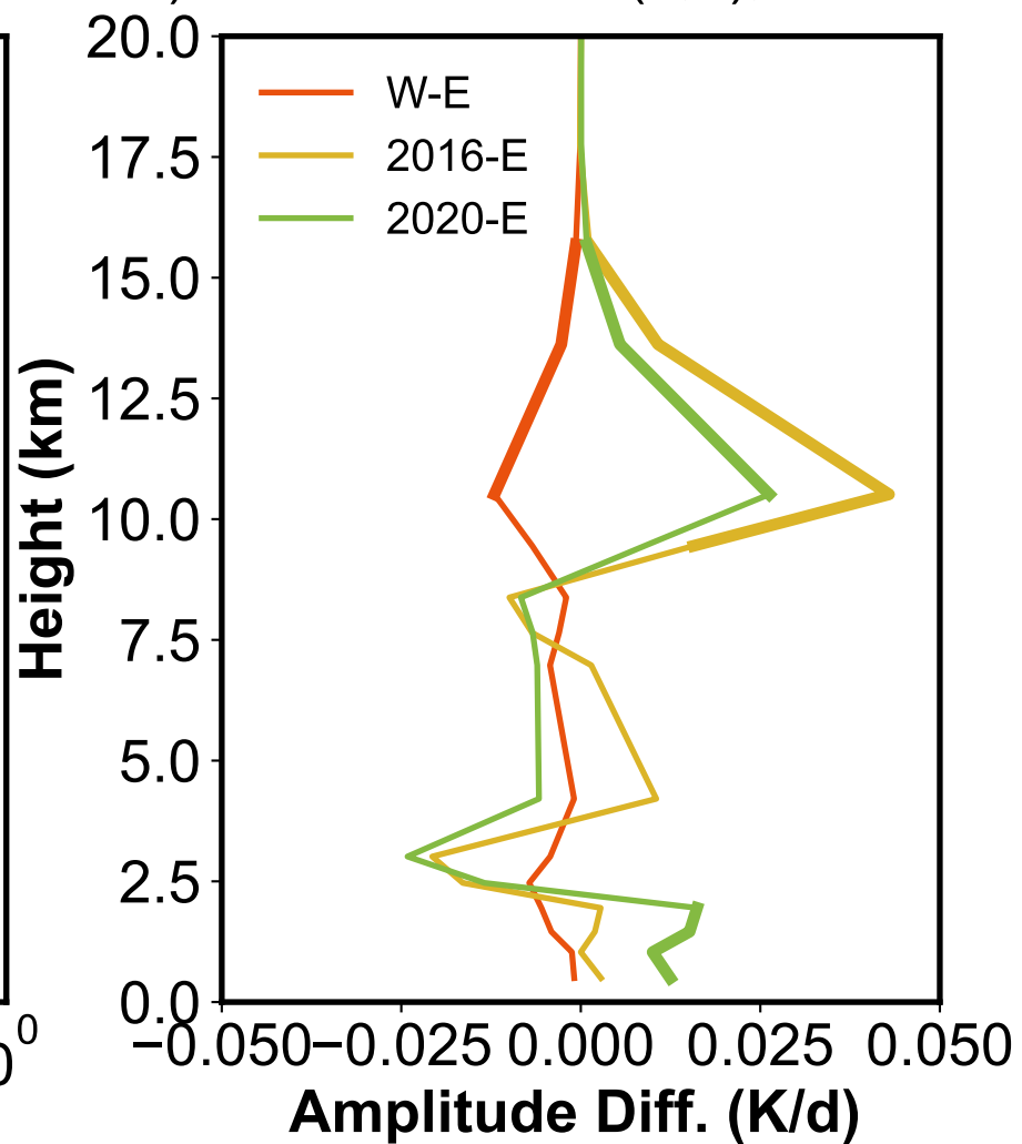
b) Difference H2O (1,1), MERRA2
