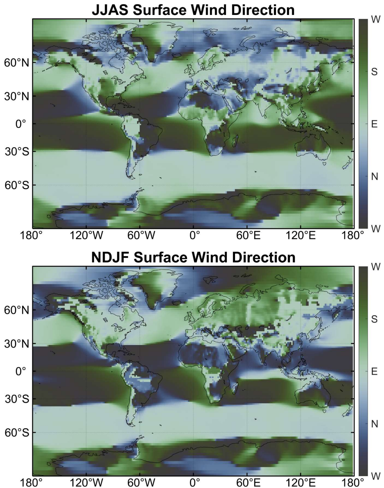
Figure S1. Average surface wind direction from ERA5 climatological reanalyses. The top panel has the average direction from June – September, and the bottom has the average direction from November – February.
