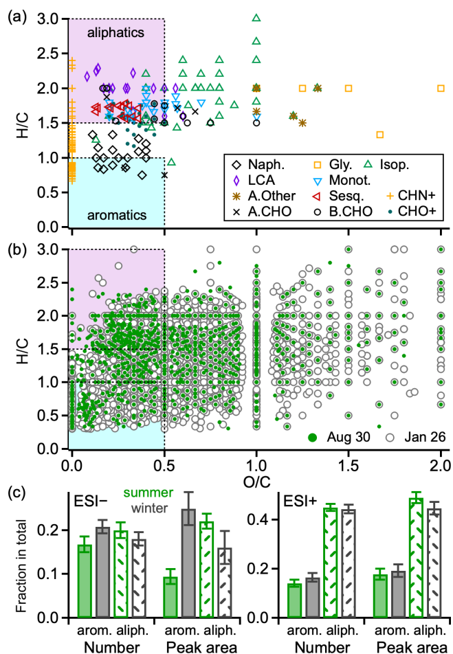
Figure 8. van Krevelen diagrams plotting of (a) organic tracer species derived from anthropogenic and biogenic precursors in both modes (as listed in Tables S1–S5), and (b) organic species identified on a summer day (30 August) and a winter day (26 January) in ESI − mode. (c) Averaged number and peak area fractions of organic species in aromatic and aliphatic molecular structures for summer and winter samples in ESI − and ESI + modes. In panels (a) and (b), the shaded pink ( H/C \geq 1.5 , O/C \leq 0.5 ) and cyan ( H/C \leq 1.0 , O/C \leq 0.5 ) areas represent aliphatic and aromatic regimes, respectively. The O/C was replaced by (O-3S)/C or (O-3S-2N)/C in the case of organosulfates or nitrooxy-organosulfates. The error bars in panel (c) represent 1\sigma standard deviations for all the samples in each season.
