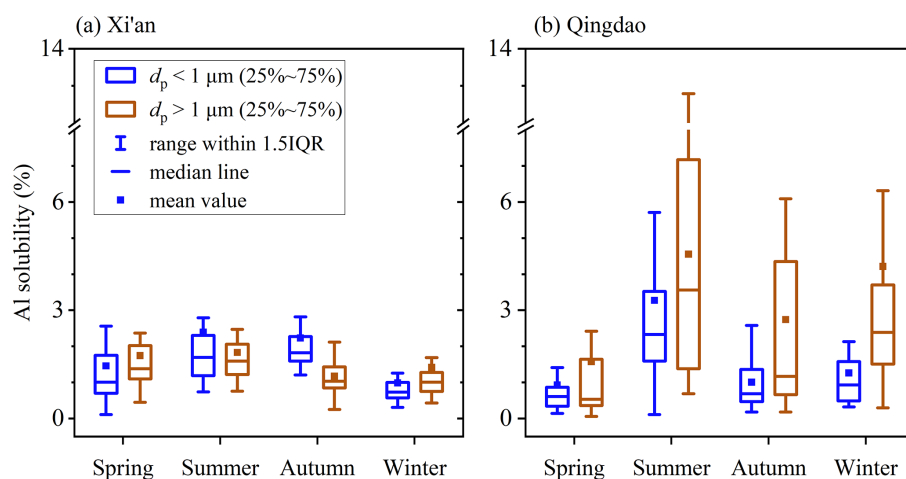
Figure 3. Seasonal variations of aerosol Al solubility for submicron and supermicron particles at (a) Xi'an and (b) Qingdao.
