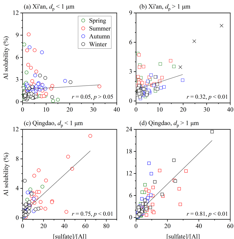
Figure 6. Aerosol Al solubility versus [\text{sulfate}]/[\text{Al}] : (a) submicron particles at Xi'an, (b) supermicron particles at Xi'an, (c) submicron particles at Qingdao, (d) supermicron particles at Qingdao (the r value changed from 0.81 to 0.74 if the data point with the highest Al solubility was excluded). Data represented by crosses are not included in fitting.
