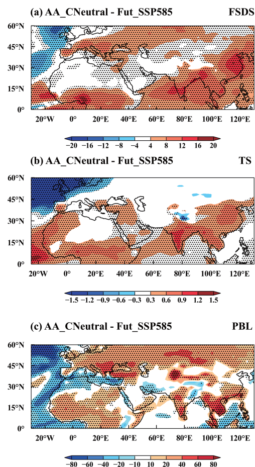
Figure 7. Spatial distribution of changes in March–May mean (a) downwelling solar flux at the surface (FSDS, \text{W m}^{-2} ), (b) surface temperature (TS, K), and (c) planetary boundary layer height (PBL, m), in 2060 for AA_CNeutral, compared to the Fut_SSP585 simulation. The stippled areas indicate statistically significant differences at the 90 % confidence level based on a two-tailed Student’s t test.
