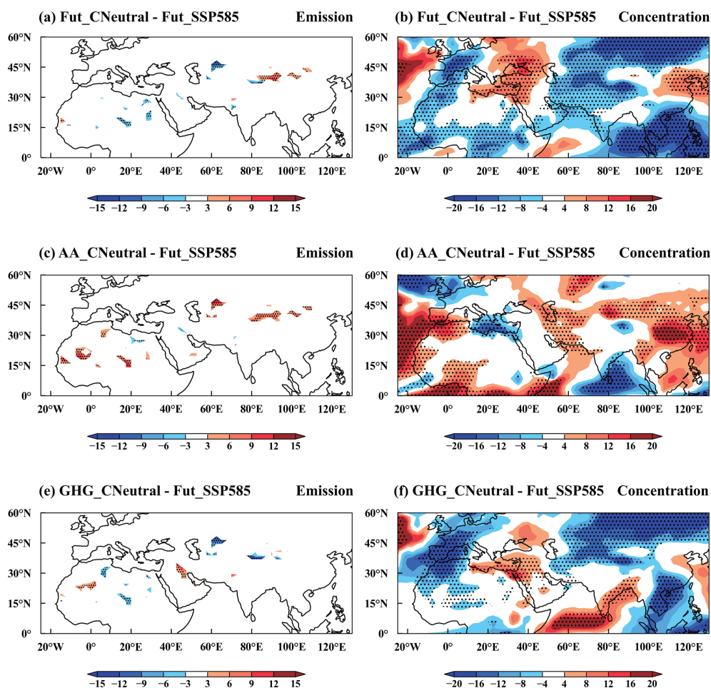
Figure 4. Spatial distribution of percentage changes in March–May mean (a, c, e) dust emissions (%) and (b, d, f) near-surface dust concentrations (%) in 2060 for Fut_CNeutral (a, b), AA_CNeutral (c, d), and GHG_CNeutral (e, f) compared to the Fut_SSP585 simulation. The stippled areas indicate statistically significant differences at the 90 % confidence level based on a two-tailed Student's t -test.
