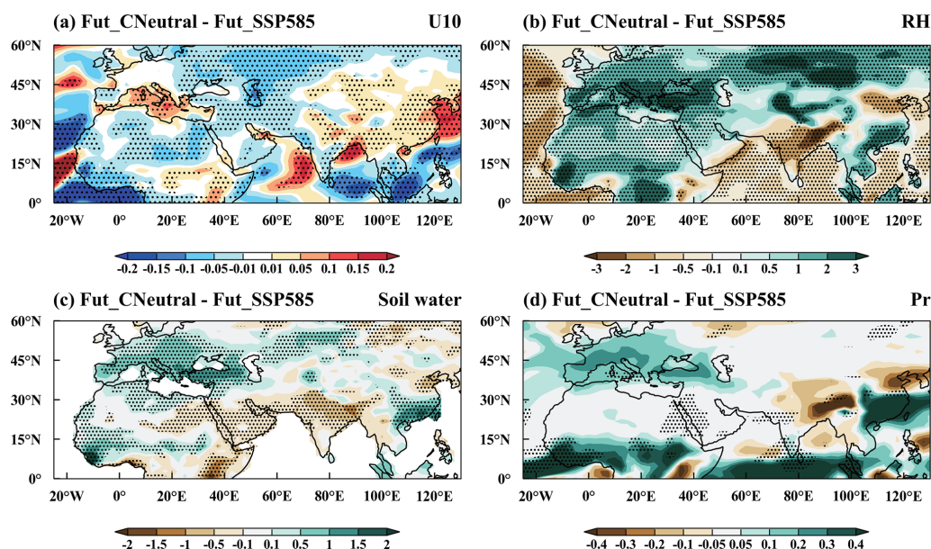
Figure 12. Spatial distribution of changes in March–May mean (a) 10 m wind speed ( U10 , \text{m s}^{-1} ), (b) relative humidity (RH, %), (c) soil water content (soil water, \text{kg m}^{-2} ), and (d) precipitation rate (pr, \text{mm d}^{-1} ) in 2060 for Fut_CNeutral, compared to the Fut_SSP585 simulation. The stippled areas indicate statistically significant differences at the 90 % confidence level based on a two-tailed Student's t test.
