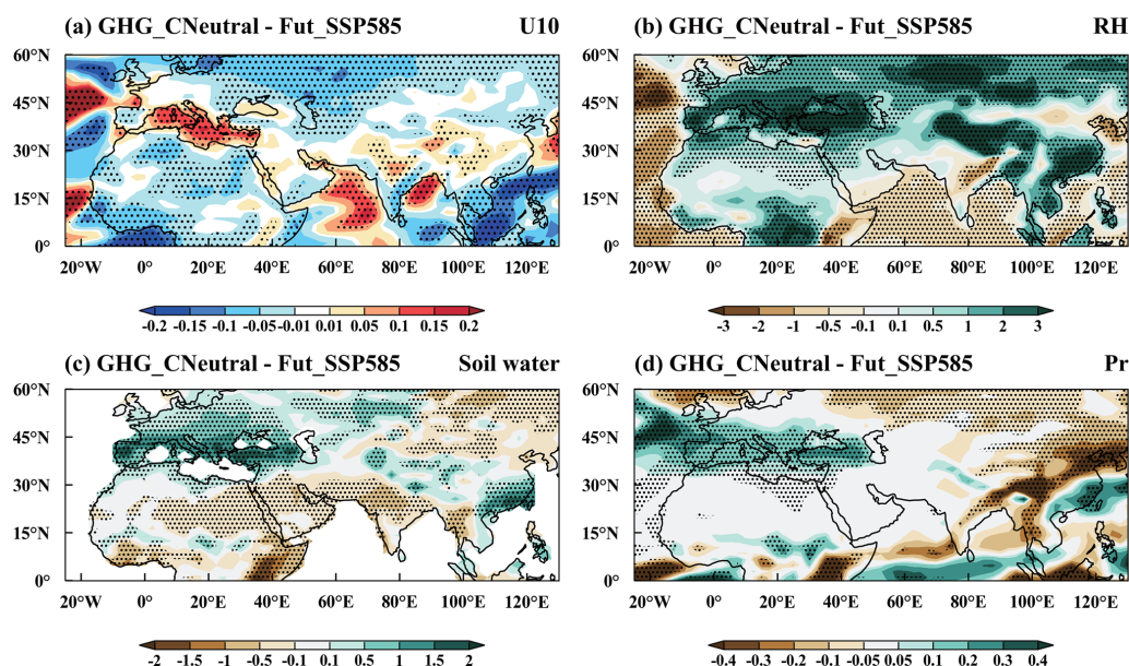
Figure 10. Spatial distribution of changes in March–May mean (a) 10 m wind speed ( U10 , \text{m s}^{-1} ), (b) relative humidity (RH, %), (c) soil water content (soil water, \text{kg m}^{-2} ), and (d) precipitation rate (pr, \text{mm d}^{-1} ) in 2060 for GHG_CNeutral, compared to the Fut_SSP585 simulation. The stippled areas indicate statistically significant differences at the 90 % confidence level based on a two-tailed Student's t test.
