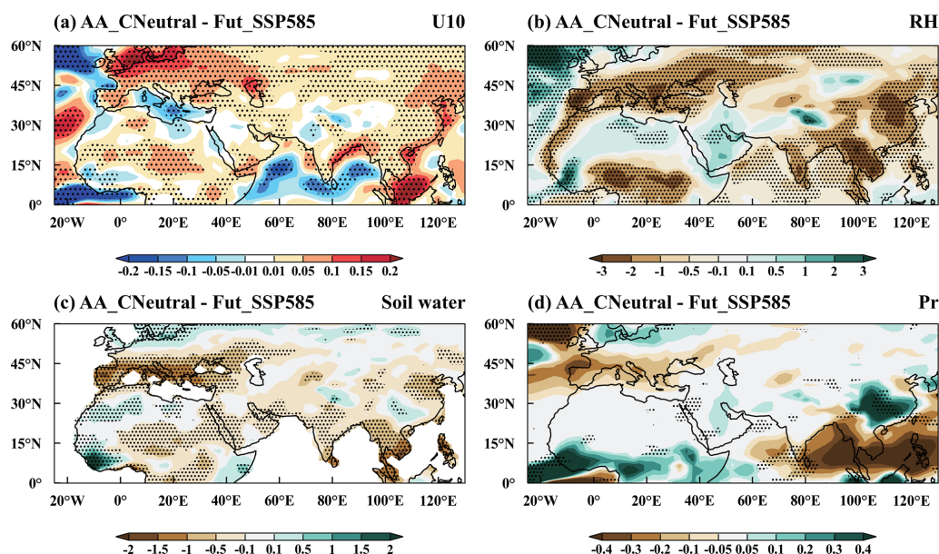
Figure 8. Spatial distribution of changes in March–May mean (a) 10 m wind speed ( U_{10} , \text{m s}^{-1} ), (b) relative humidity (RH, %), (c) soil water content (soil water, \text{kg m}^{-2} ), and (d) precipitation rate (pr, \text{mm d}^{-1} ) in 2060 for AA_CNeutral, compared to the Fut_SSP585 simulation. The stippled areas indicate statistically significant differences at the 90 % confidence level based on a two-tailed Student's t test.
