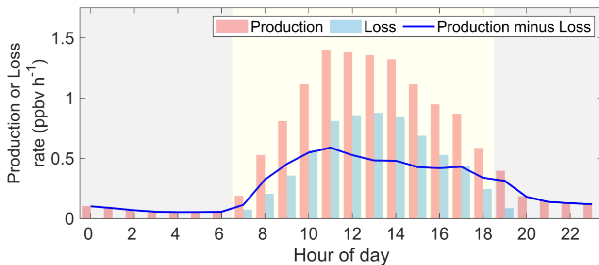
Figure S4. The diurnal variations of the simulated chemical production, loss, and their difference (production minus loss) rate of HONO.
