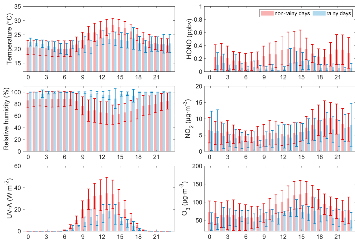
Figure S2. Diurnal variations of the observed meteorological parameters (air temperature, relative humidity, UV-A radiation) and air pollutants (HONO, NO 2 , O 3 ) on rainy and non-rainy days during the study period.
