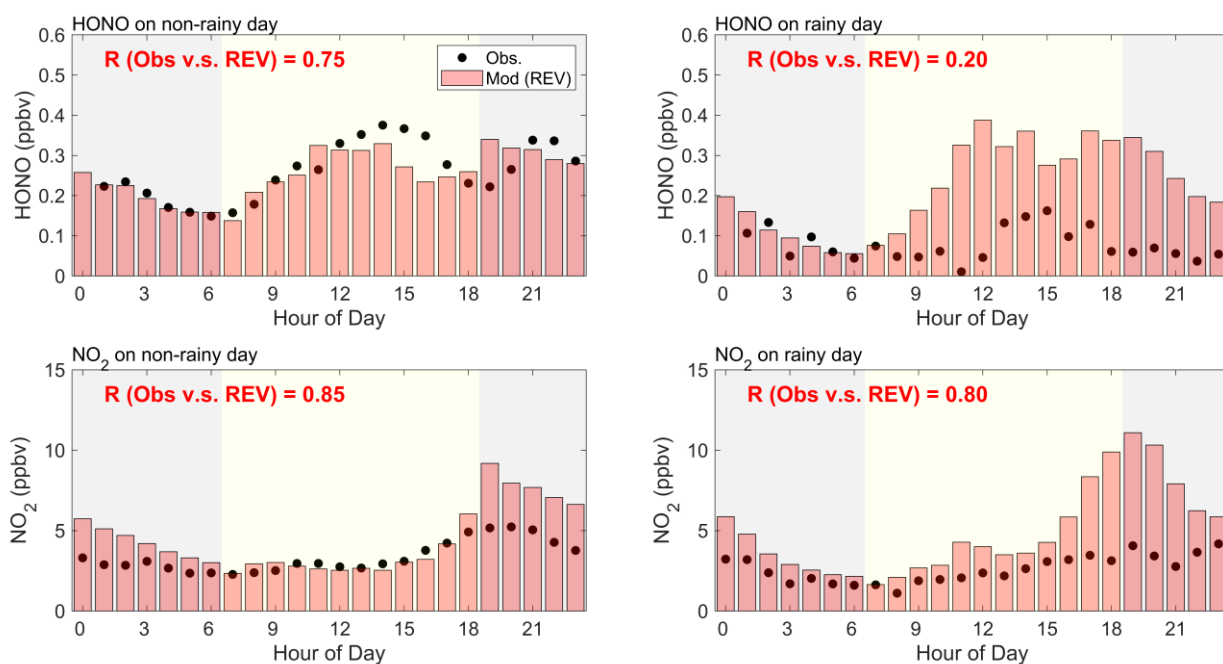
Figure S3. The diurnal variations of the observed and simulated HONO and NO 2 concentrations on rainy days and non-rainy days.
