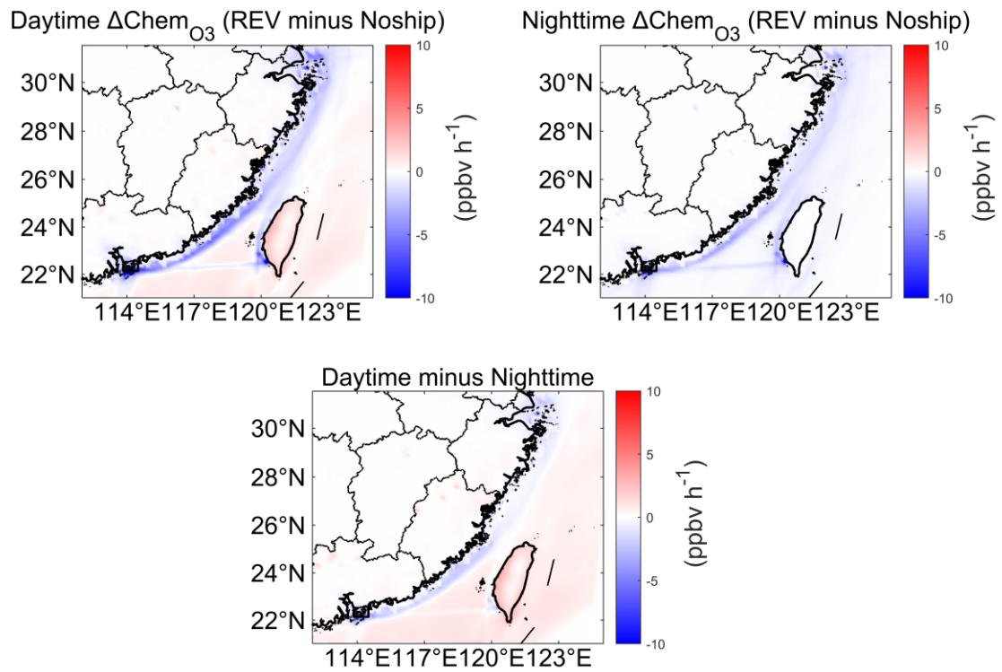
Figure S7. Spatial distribution of impacts of shipping emissions on chemical production rates of O 3 ( \Delta\text{Chem}_{\text{O}_3} ) during the daytime and nighttime (upper panels). The difference between the daytime and nighttime is also presented in the bottom panel.
