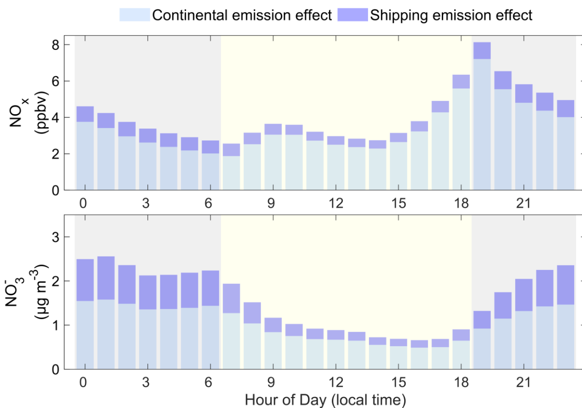
Figure S6. Diurnal variations of contributions of continental and shipping emissions to \text{NO}_x and nitrate aerosol concentrations in the coastal regions of Fujian.
