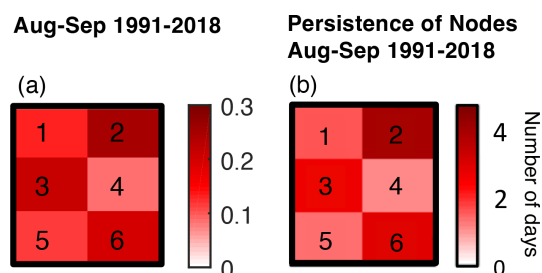
Figure 2. (a) August to September circulation regimes of occurrence for the six nodes displayed in Fig. 1; calculated for all years from 1991 to 2018, (b) the mean persistence of nodes (in days).
