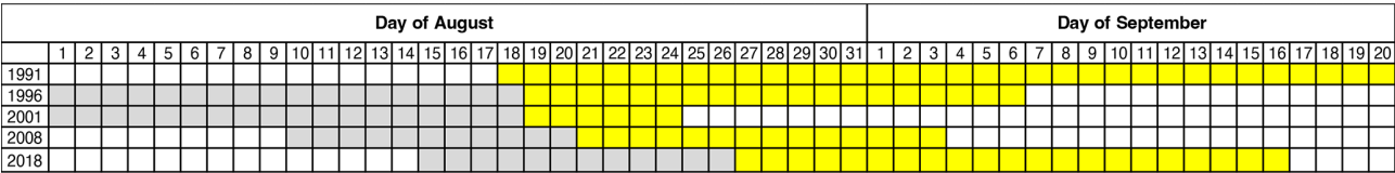
Figure A1. Overview of available number-size distributions of aerosol particles measured on I/B Oden during five Arctic expeditions, covering days in August and September in 1991, 1996, 2001, 2008, and 2018. Gray days represent “melt”, and yellow days represent “freeze-up”. White fields indicate days without data.
