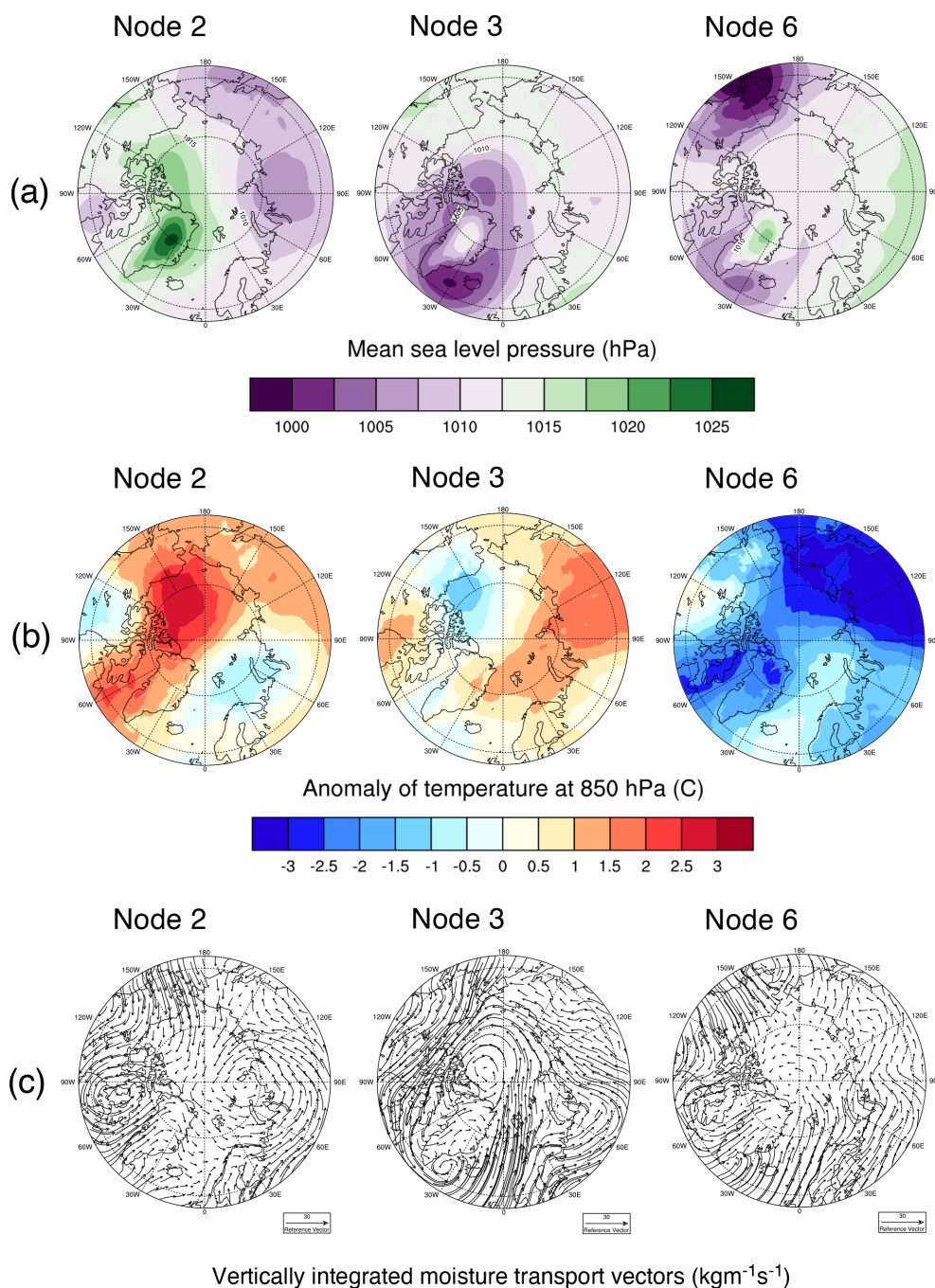
Figure 3. (a) Mean sea-level pressure in hPa, (b) the anomaly of temperature in °C for 850 hPa, (c) vertically integrated moisture transport vectors in \text{kg m}^{-1} \text{s}^{-1} for circulation regimes (nodes) 2, 3, and 6; were calculated for August–September, including all years from 1991 to 2018.
