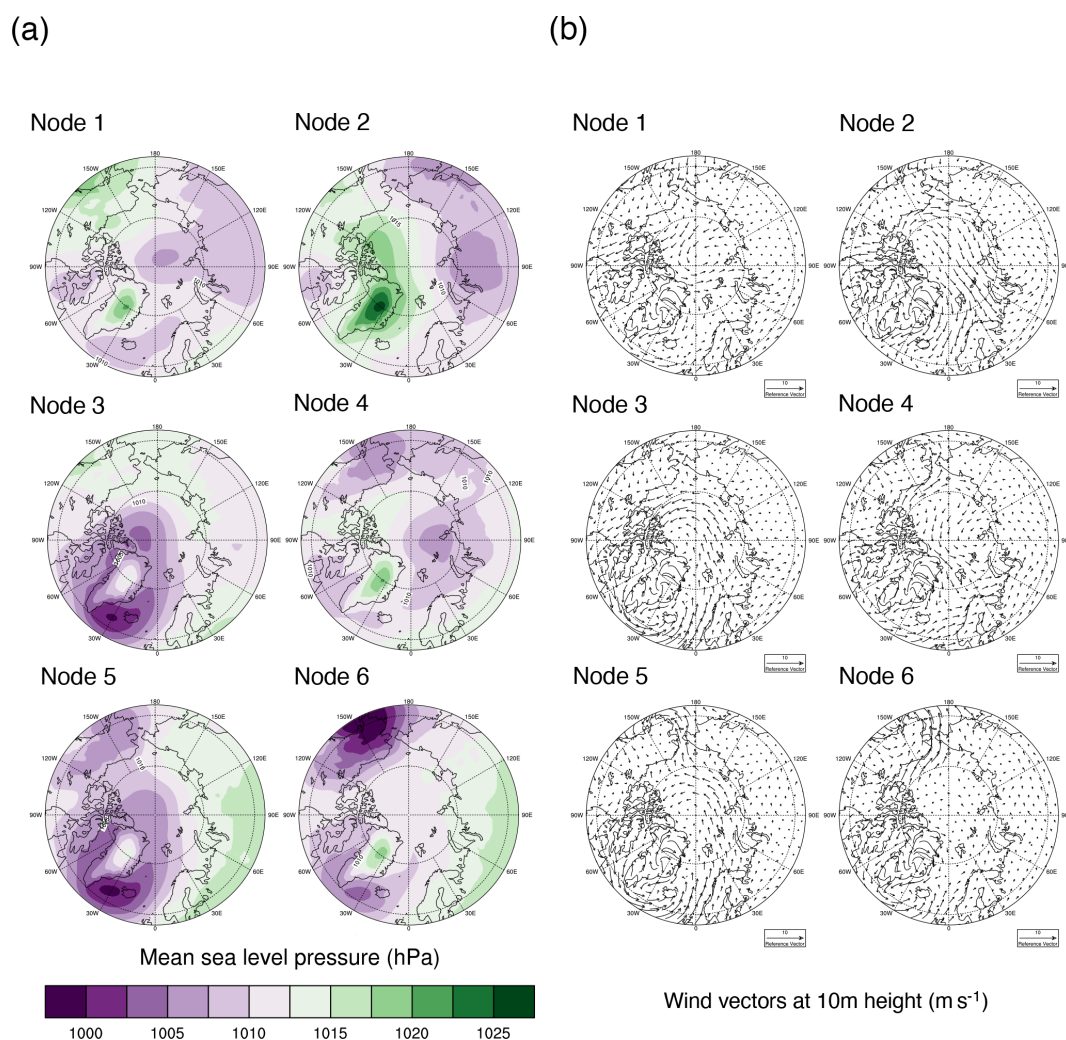
Figure 1. (a) Mean sea-level pressure and (b) wind vector at 10 m height above ground level circulation regimes ( 2 \times 3 nodes): calculated for August–September, including all years from 1991 to 2018.
