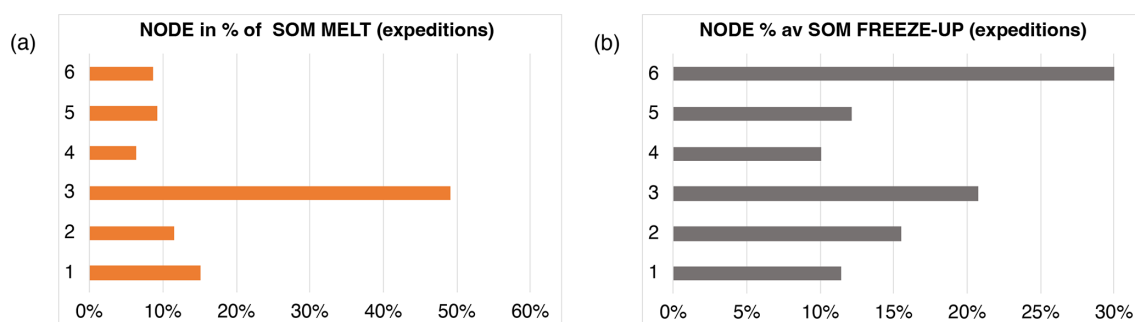
Figure 6. Probabilities of the occurrence of the six nodes in Fig. 2 in August and September for the five expedition years: 1991, 1996, 2001, 2008, and 2018. The data is sorted into (a) “melt” and (b) “freeze-up”.
