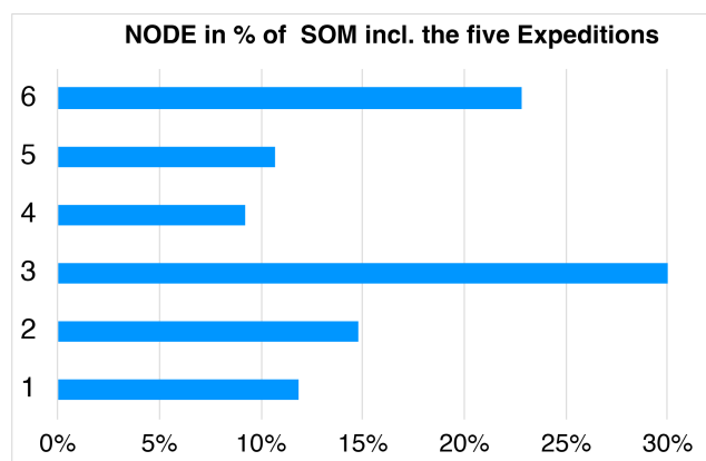
Figure 5. Probabilities of the occurrence of the six nodes in Fig. 2 in August and September for the five expedition years: 1991, 1996, 2001, 2008, and 2018.
