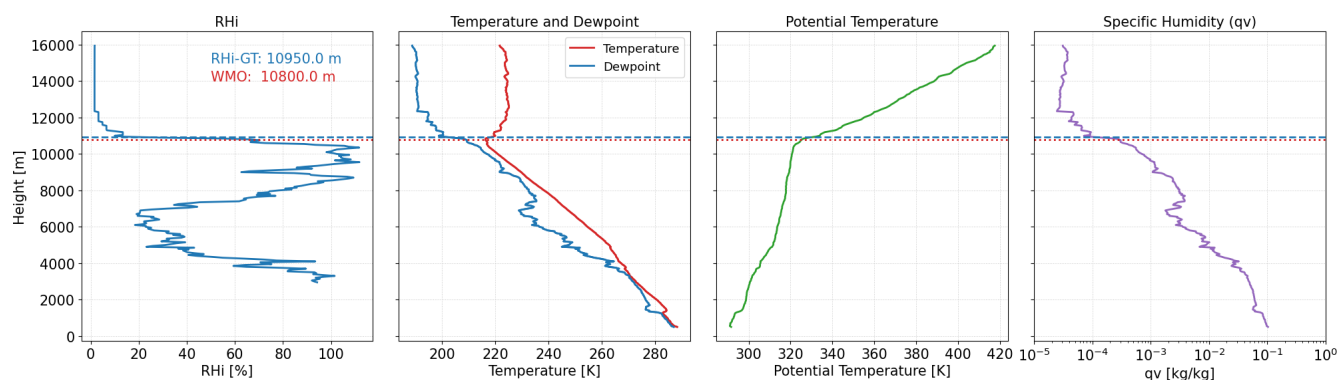
Figure 1. Vertical profile of RHi, temperature (red), dew point (blue), potential temperature and specific humidity of the radiosonde ascent from Meiningen, 2 June 2024, 12:00 UTC. RHi values are shown for temperatures below 273.15 K. The RHi-GT level (blue-dashed) and thermal tropopause level (red-dotted) are shown in every subplot.
