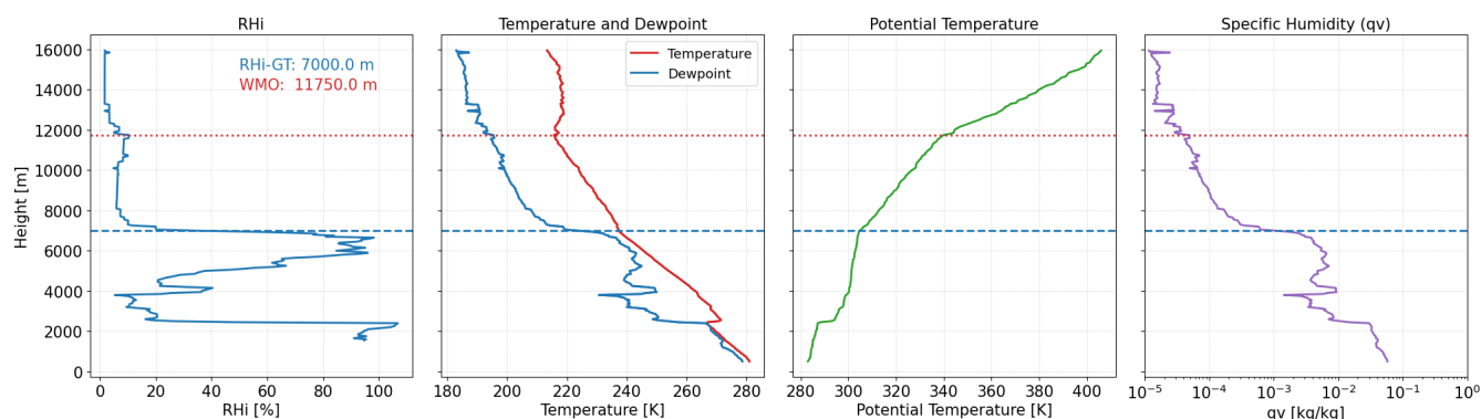
Figure 2. Same as Fig. 1, but for 18 February 2024, 00:00 UTC.
