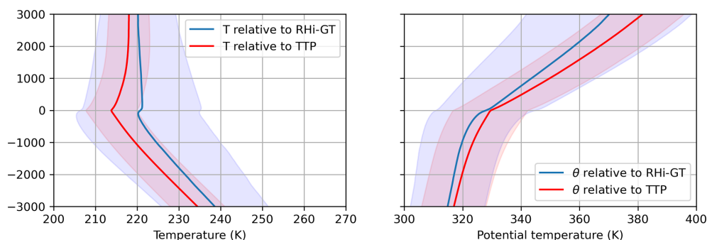
Figure 6. Mean of the (left) absolute temperature and (right) potential temperature relative to the tropopause. Blue color denotes the results for the RHi-GT, while red colors denote the results relative to the TTP. Shading denotes the range of the standard deviation.
