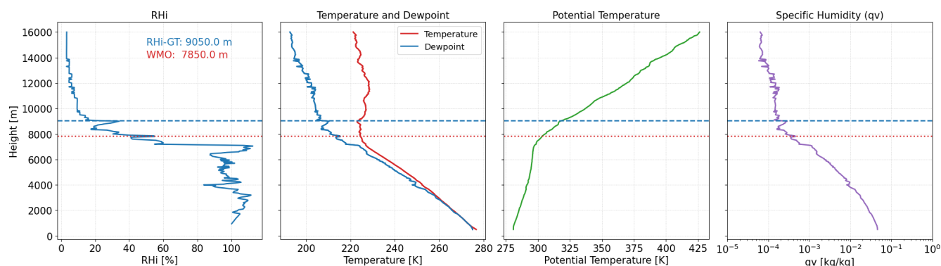
Figure 3. Same as Fig. 1, but for 20 April 2024, 00:00 UTC.
