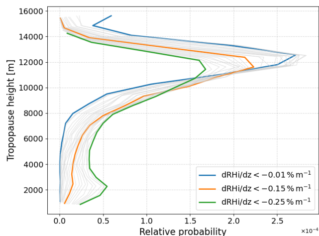
Figure 9. Tropopause height histogram depending on the choice of the vertical RHi gradient for the 10 year time period. The weakest vertical RHi gradient threshold of -0.01 \text{ m}^{-1} is shown in blue, the RHi gradient used for the previous evaluation in this study of -0.15 \text{ m}^{-1} is shown in orange. In green the strongest RHi gradient of -0.25 \text{ m}^{-1} used in this sensitivity evaluation is shown. The values in between are displayed in grey in increments of 0.01 \text{ m}^{-1} .
