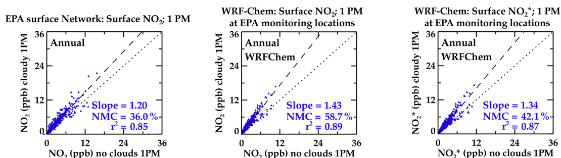
Figure 6. Scatterplots intercomparing annualized surface NO 2 at 13:30 local time during cloudy days vs. cloud free days. (Left) EPA AQS data which is a repeat of Fig. 3c. (Center) WRF-Chem collocated with the AQS monitoring sites, and using the WRF-Chem cloud filter in lieu of the TROPOMI cloud filter. (Right) WRF-Chem collocated with the AQS monitoring sites, comparing NO 2 * instead of NO 2 .
