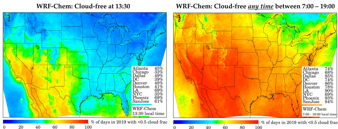
Figure 2. Percentage of days over the contiguous US during 2019 with cloud fractions less than 0.5 as simulated by WRF-Chem at various local times: (Left) 13:30, (Right) any time between 07:00–19:00.
