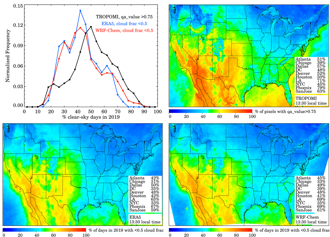
Figure 1. Percentage of clear-sky days over the contiguous US during 2019 from the TROPOMI NO 2 V2.4 product, ERA5 re-analysis, and WRF-Chem. (Top left) Normalized frequency diagram of the binned percentage of clear sky days for the three products. (Top right) Percentage of days in which the qa_value of the TROPOMI NO 2 V2.4 measurement was greater than 0.75. (Bottom left) Percentage of days in which the total cloud cover (tcc) from the ERA5 was less than 0.5. (Bottom right) Percentage of days in each grid cell in which the total cloud fraction from the WRF-Chem was less than 0.5.
