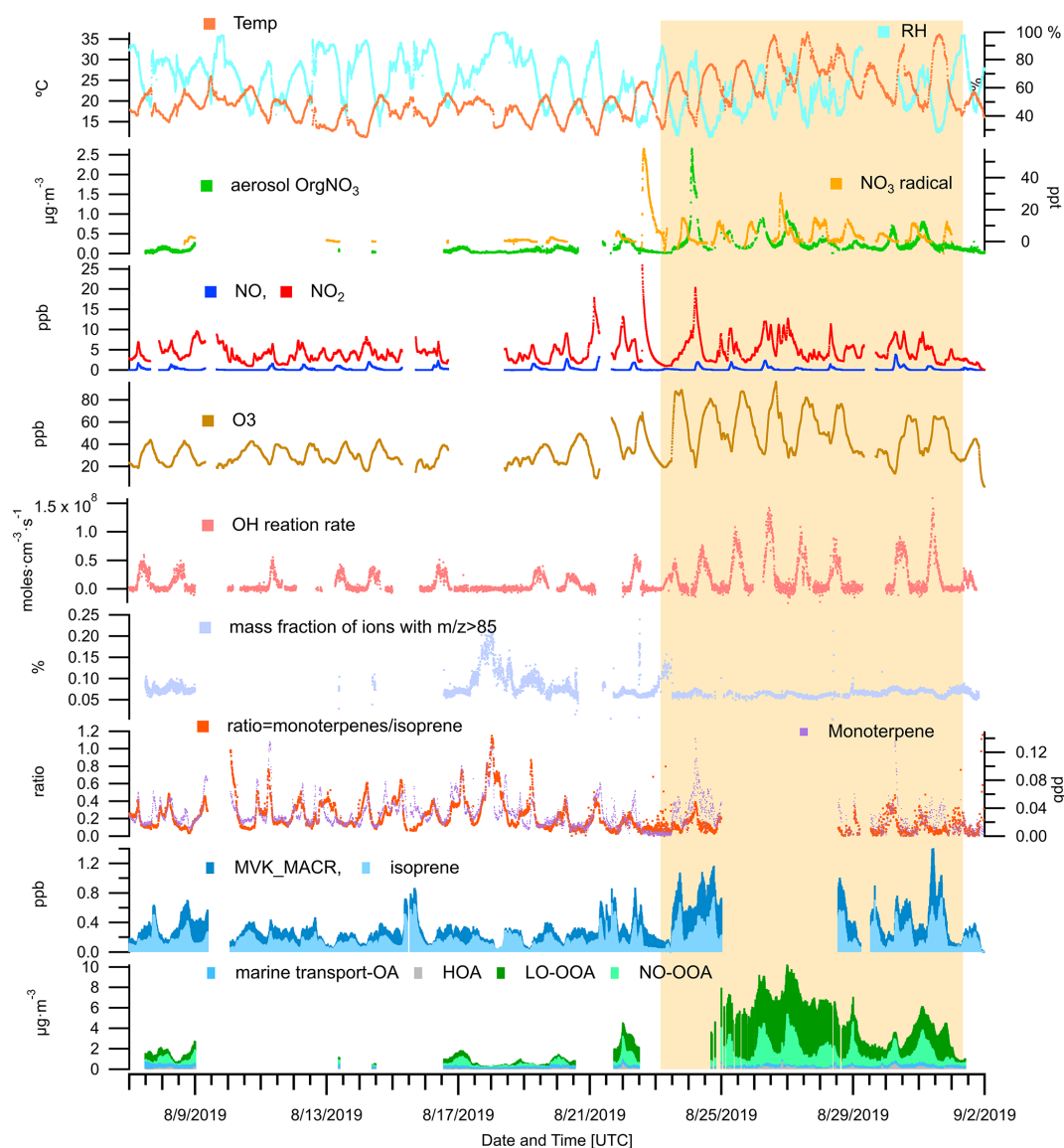
Figure 13. An overview of OA source contributions, ambient measurements of trace gases (VOCs, \text{O}_3 , \text{NO}_x , \text{N}_2\text{O}_5 , \text{NO}_3 radicals), meteorological parameters (temperature and RH), and calculated parameters are provided for the JULIAC summer period. The calculated parameters include the OH reaction rate (derived from measured OH concentrations and OH reactivity), the mass fraction of ions with m/z > 85 in OA measured by the ToF-AMS, and the concentration ratio of monoterpenes to isoprene. The period of the heatwave event observed in summer is highlighted with a yellow background.
