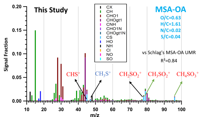
Figure 8. MSA-OA factor profile of this study. Typical MSA marker fragments: \text{CHS}^+ ( m/z 44.98), \text{CH}_3\text{S}^+ ( m/z 47.00), \text{CH}_2\text{SO}_2^+ ( m/z 77.98), \text{CH}_3\text{SO}_2^+ ( m/z 78.99), and \text{CH}_4\text{SO}_3^+ ( m/z 95.99) are highlighted in the factor profile. Normalized ion attribution is colored by corresponding ion family groups, and elemental ratios (O/C, H/C, N/C, S/C) of the MSA-OA factor are also marked in the graph. The y axis presents the ion signal intensity fraction.
