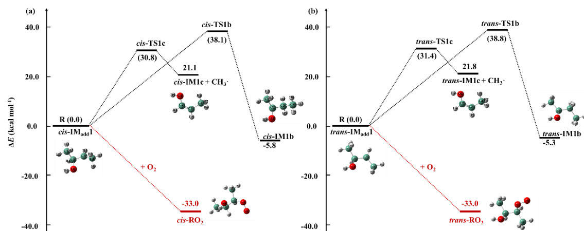
Figure S4. PESs for the reaction of (a) cis -IM add 1 and (b) trans -IM add 1 predicted at the DLPNO-CCSD(T)/aug-cc-pVTZ//M06-2X/6-311+G(2df,2p) level of theory (in kcal mol -1 ).
