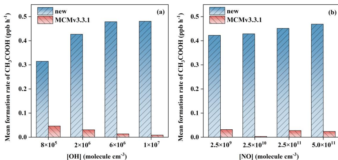
Figure S10. Mean formation rate of \text{CH}_3\text{COOH} (unit: \text{ppb h}^{-1} ) from the trans -BU + OH reactions as a function of (a) OH concentration ( [\text{OH}] ) and (b) NO concentration ( [\text{NO}] ) under the petrochemical region conditions. The comparison is made between the MCM v3.3.1 and the new mechanism.
