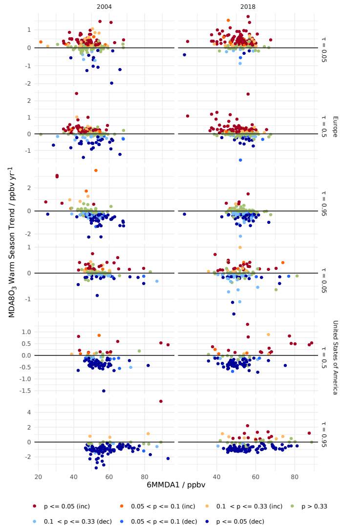
Figure S23: For the years 2004 (left) and 2018 (right) scatter plots show that years' warm season MDA8O 3 trend in (top to bottom) Europe \tau = 0.05, 0.5, 0.95 , United States of America \tau = 0.05, 0.5, 0.95 vs the 6MMDA1 for the same year. Colours show significance of trend.
