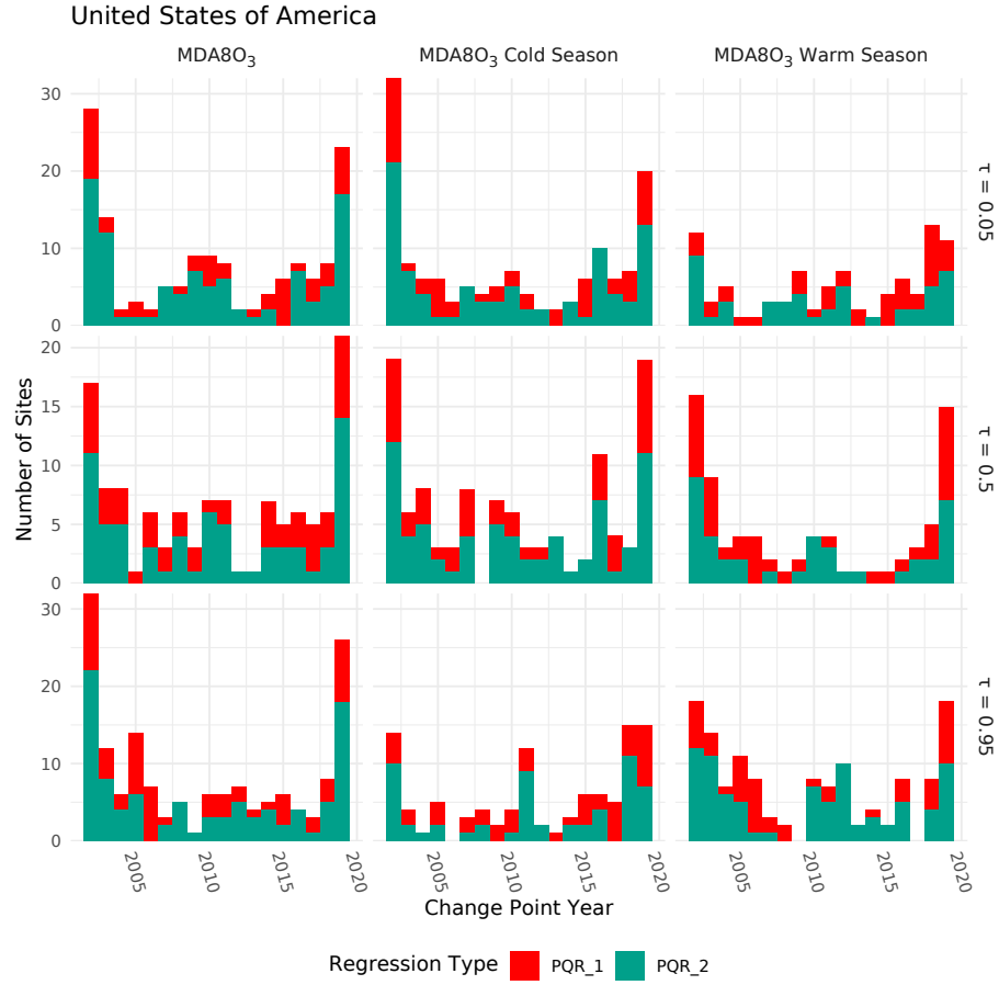
Figure S2: Years where change points have been assigned in MDA8O 3 all, cold and warm season (left to right) for sites in the USA. Top to bottoms shows \tau = 0.05, 0.5, 0.95 . Stacked areas separate change points by PQR_1 (red) and PQR_2 (green)
