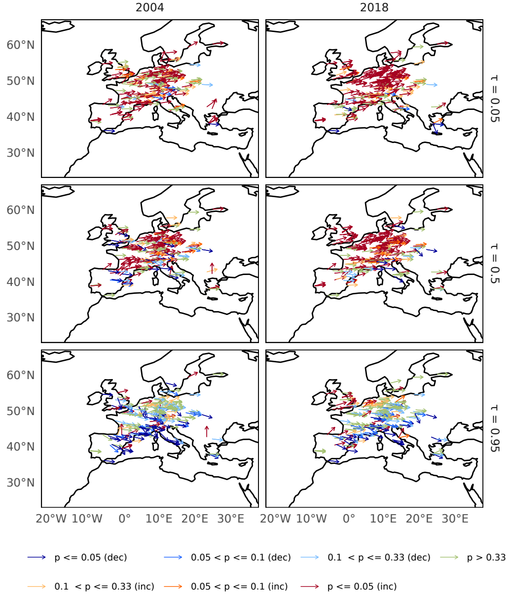
Figure S6: Trends in MDA8O 3 in Europe in 2004 (left) and 2018 (right). Trends are shown by an arrow where the angle between vertically up and horizontal corresponds to 2.5 - 0 ppbv / yr -1 , and between horizontal and vertically down corresponds to 0 - -2.5 ppbv / yr -1 . The few trends that have a magnitude greater than 2.5 ppbv have been clamped. Colour corresponds to the direction and significance of the trend.
