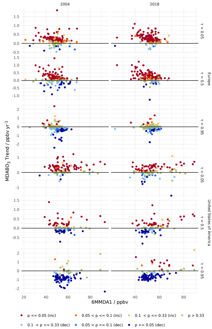
Figure S22: For the years 2004 (left) and 2018 (right) scatter plots show that years' MDA8O 3 trend in (top to bottom) Europe \tau = 0.05, 0.5, 0.95 , United States of America \tau = 0.05, 0.5, 0.95 vs the 6MMDA1 for the same year. Colours show significance of trend.
