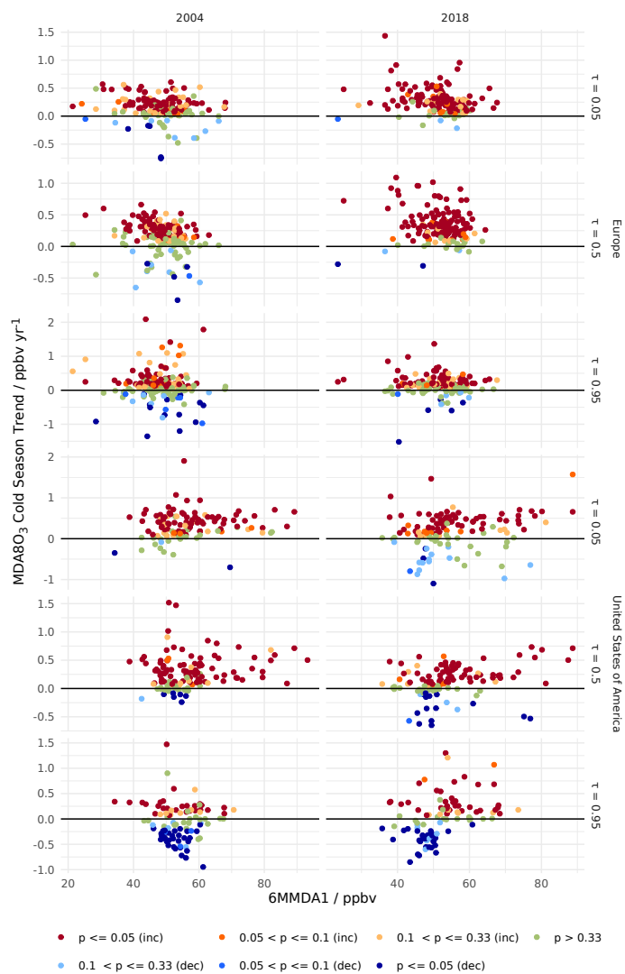
Figure S24: For the years 2004 (left) and 2018 (right) scatter plots show that years' cold season MDA8O 3 trend in (top to bottom) Europe \tau = 0.05, 0.5, 0.95 , United States of America \tau = 0.05, 0.5, 0.95 vs the 6MMDA1 for the same year. Colours show the significance of the trend.
