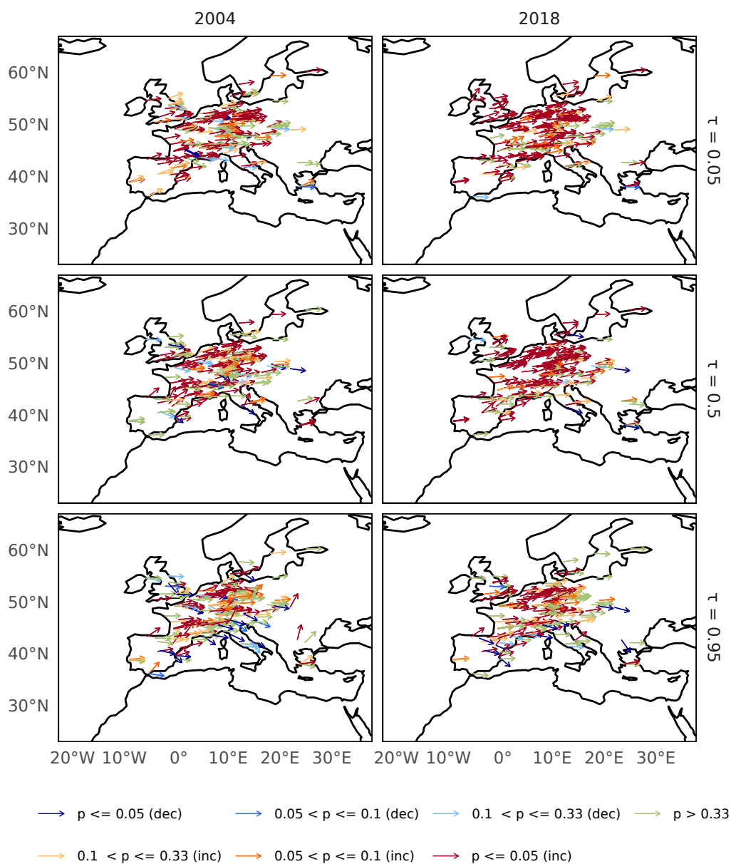
Figure S8: Trends in cold season MDA8O 3 in Europe in 2004 (left) and 2018 (right), for \tau = 0.05, 0.50 and 0.95 (top to bottom). Trends are shown by an arrow where the angle between vertically up and horizontal corresponds to 2.5 - 0 ppbv / yr -1 , and between horizontal and vertically down corresponds to 0 - -2.5 ppbv / yr -1 . The few trends that have a magnitude greater than 2.5 ppbv have been clamped. Colour corresponds to the direction and significance of the trend.
