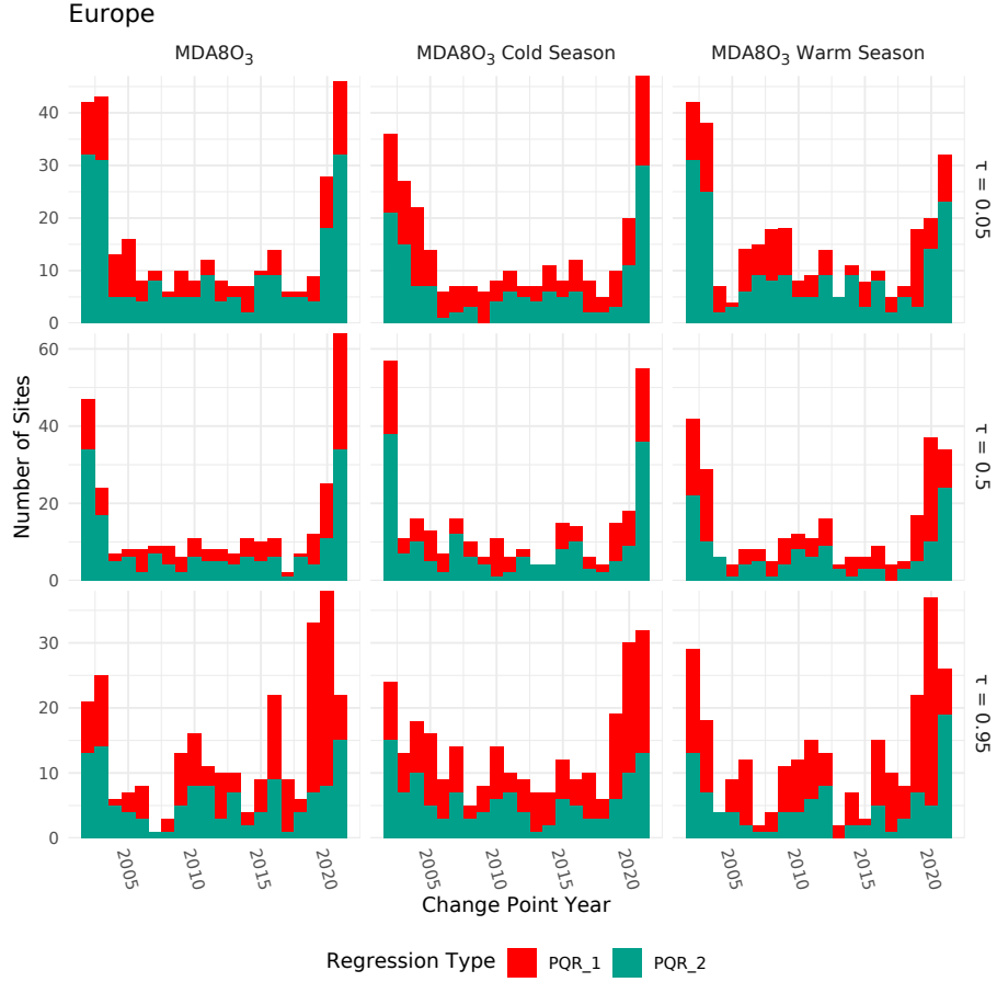
Figure S1: Years where change points have been assigned in MDA8O 3 all, cold and warm season (left to right) for sites in Europe. Top to bottoms shows \tau = 0.05, 0.5, 0.95 . Stacked areas separate change points by PQR_1 (red) and PQR_2 (green)
