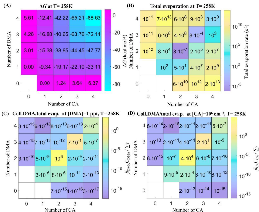
Figure S9. (A) Gibbs formation free energies ( \Delta G ) of the (CA)_{1-4}(DMA)_{1-4} clusters identified at the DLPNO-CCSD(T)/aug-cc-pVTZ// \omega B97X-D/6-31++G(d,p) level of theory, T = 258 K, p = 1 atm. (B) Total evaporation rate coefficients ( \Sigma\gamma in s^{-1} ) and the ratios of collision frequencies with (C) DMA monomer or (D) CA monomer versus total evaporation rate coefficients ( \beta_{DMA}C_{DMA}/\Sigma\gamma or \beta_{CA}C_{CA}/\Sigma\gamma ) of the corresponding clusters.
