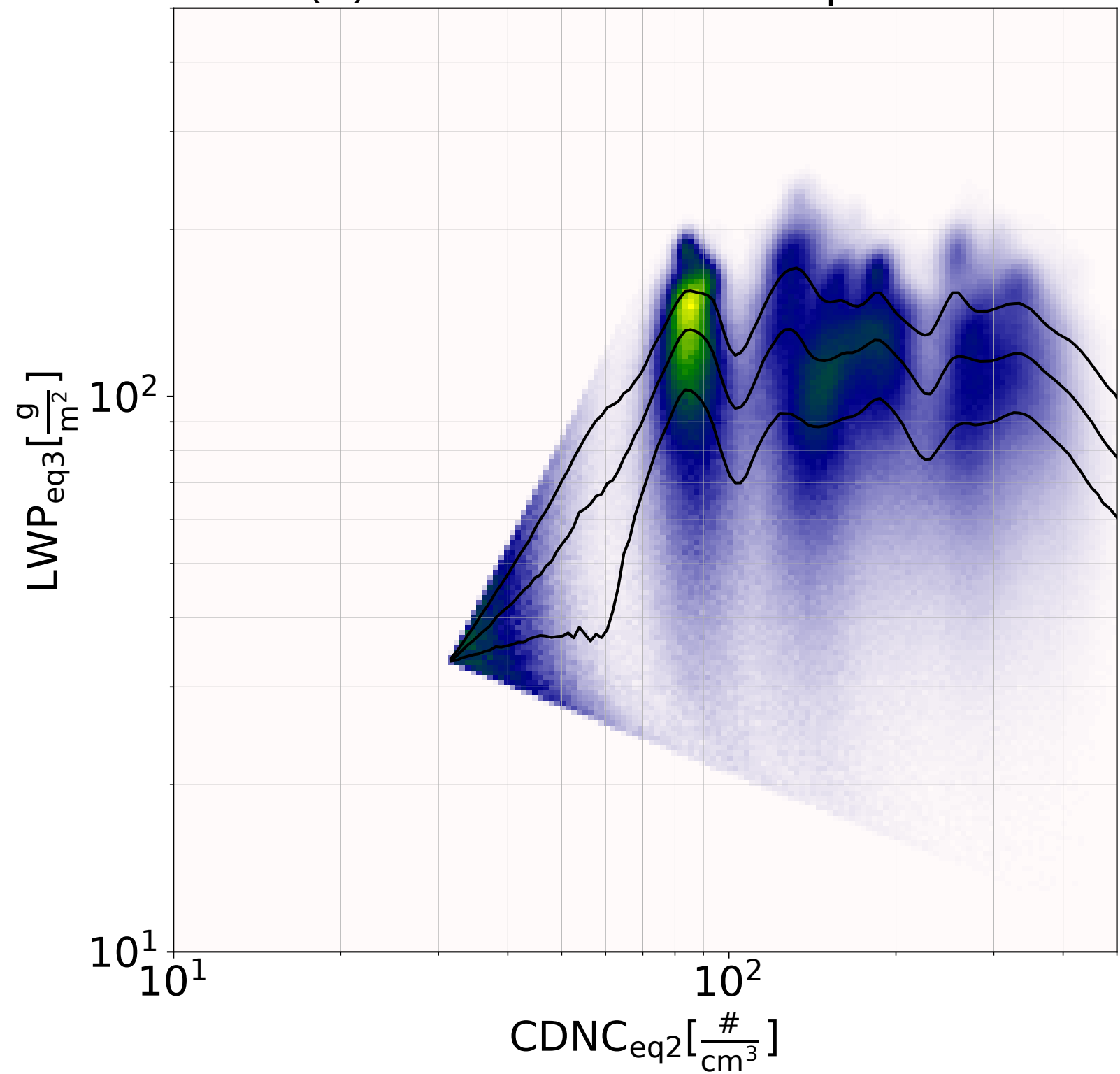
(b) Satellite retrieval equations
