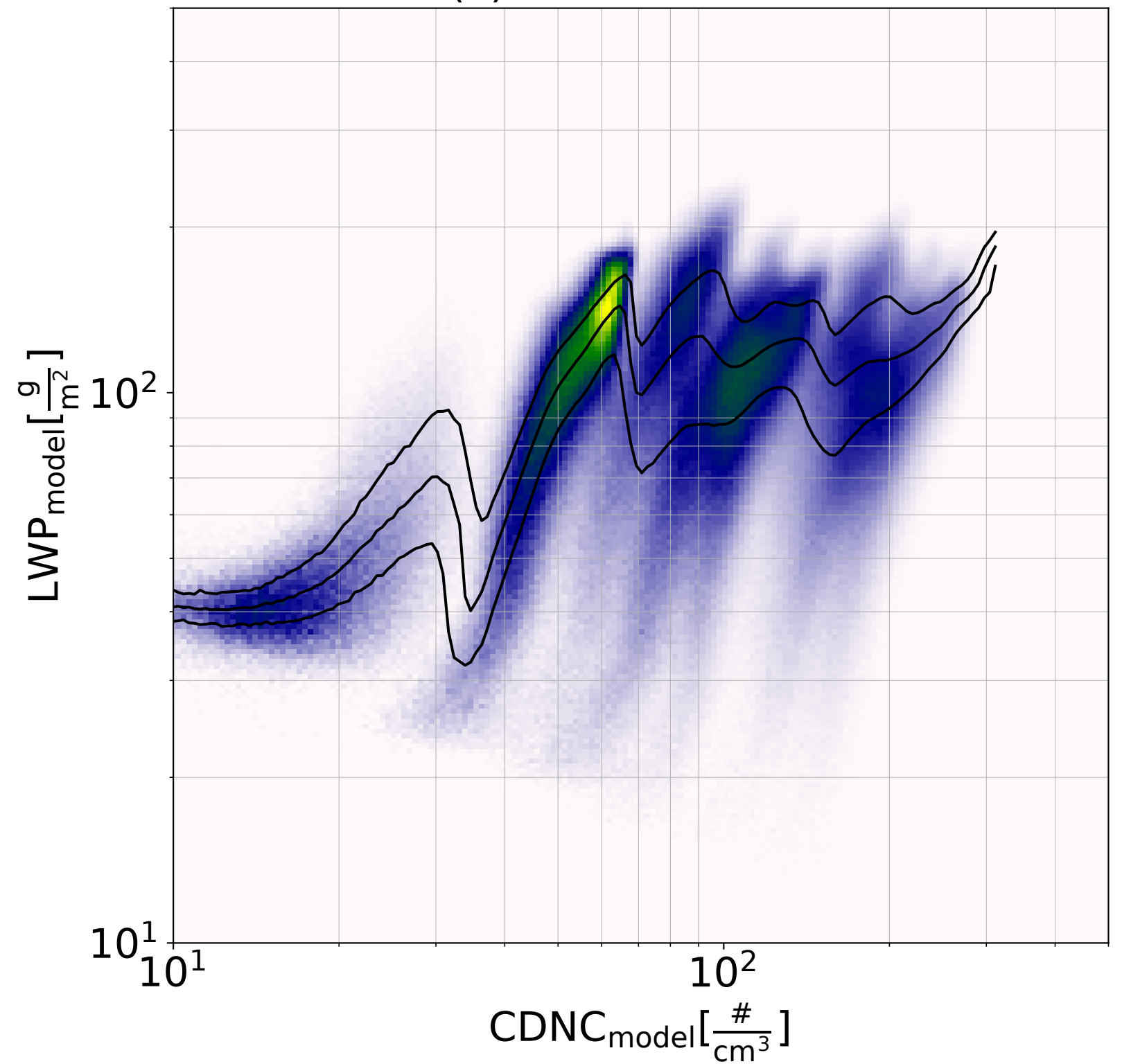
(a) UCLALES-SALSA
