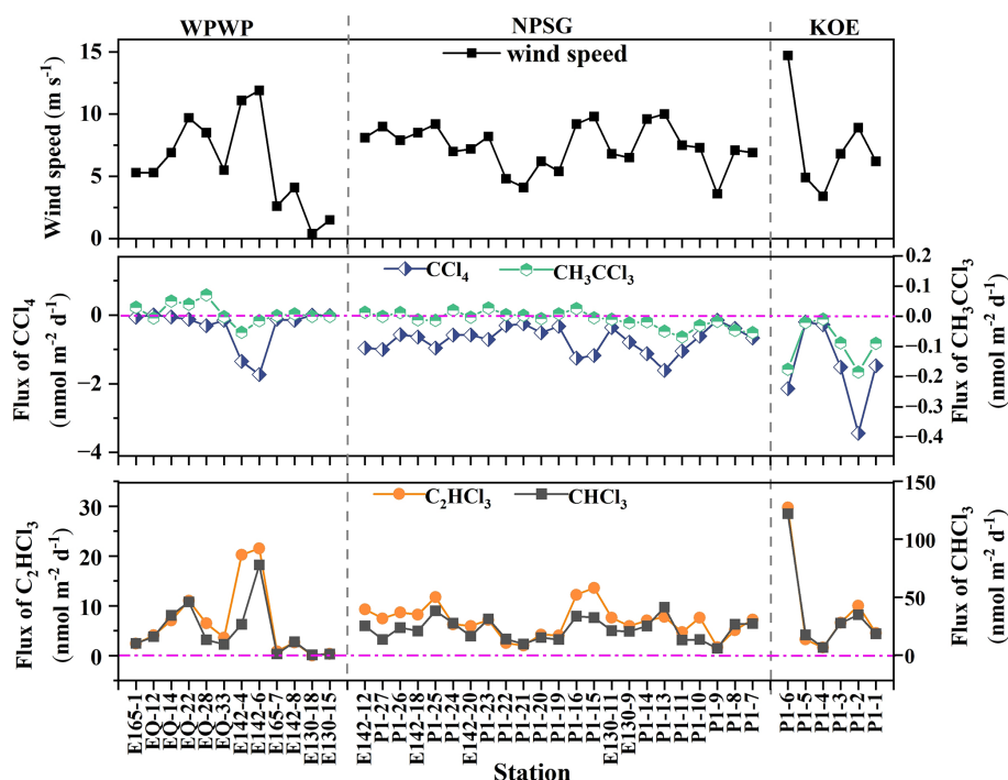
Figure 5. Sea–air fluxes of \text{CCl}_4 , \text{CH}_3\text{CCl}_3 , \text{CHCl}_3 , and \text{C}_2\text{HCl}_3 , along with wind speeds in the Western Pacific.
