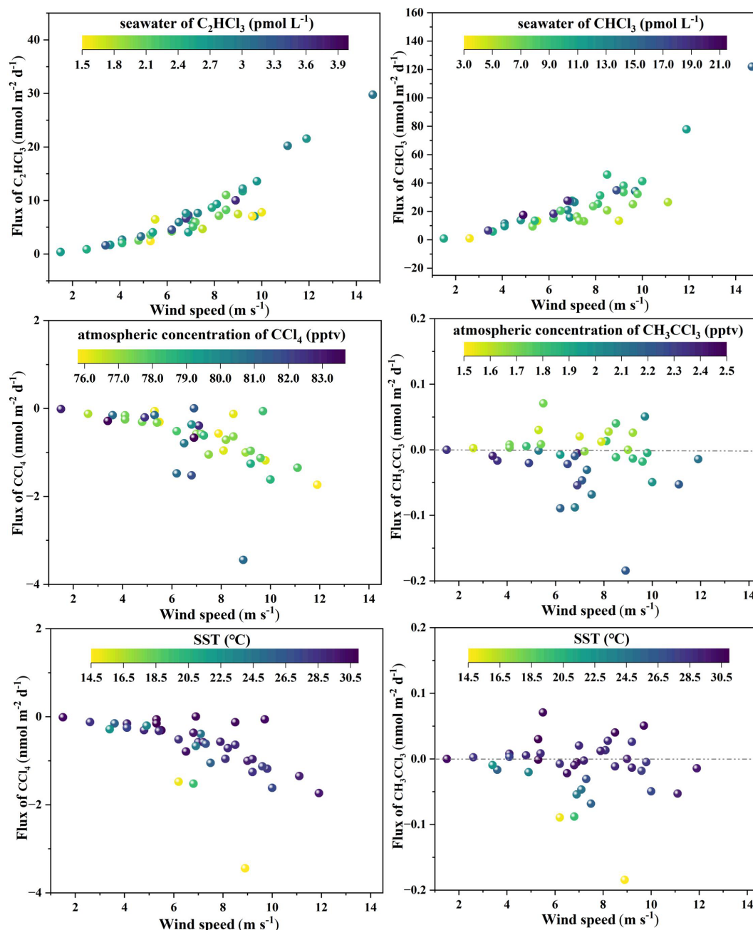
Figure 6. Relationships between sea–air fluxes of VCHCs and wind speed, SST, and VCHCs concentrations in seawater and the atmosphere.
