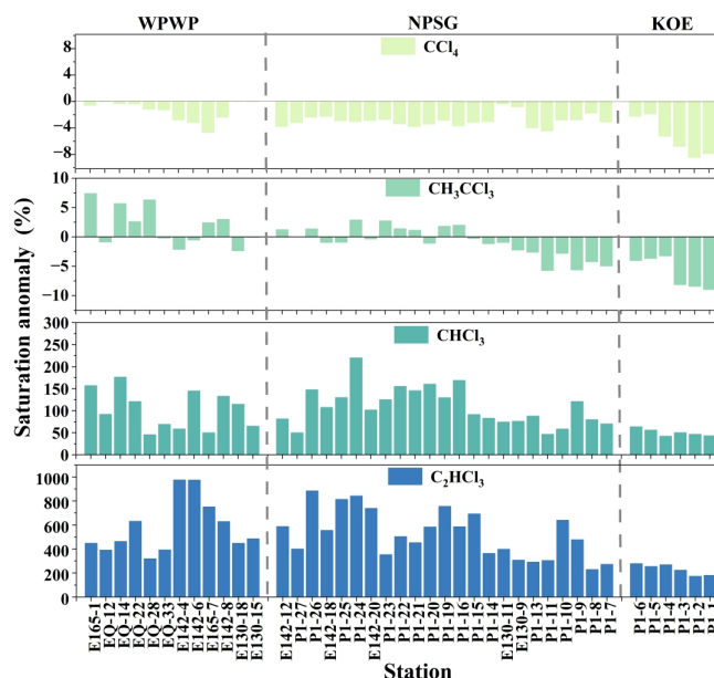
Figure 4. Saturation anomaly of \text{CCl}_4 , \text{CH}_3\text{CCl}_3 , \text{CHCl}_3 , and \text{C}_2\text{HCl}_3 in the Western Pacific.
