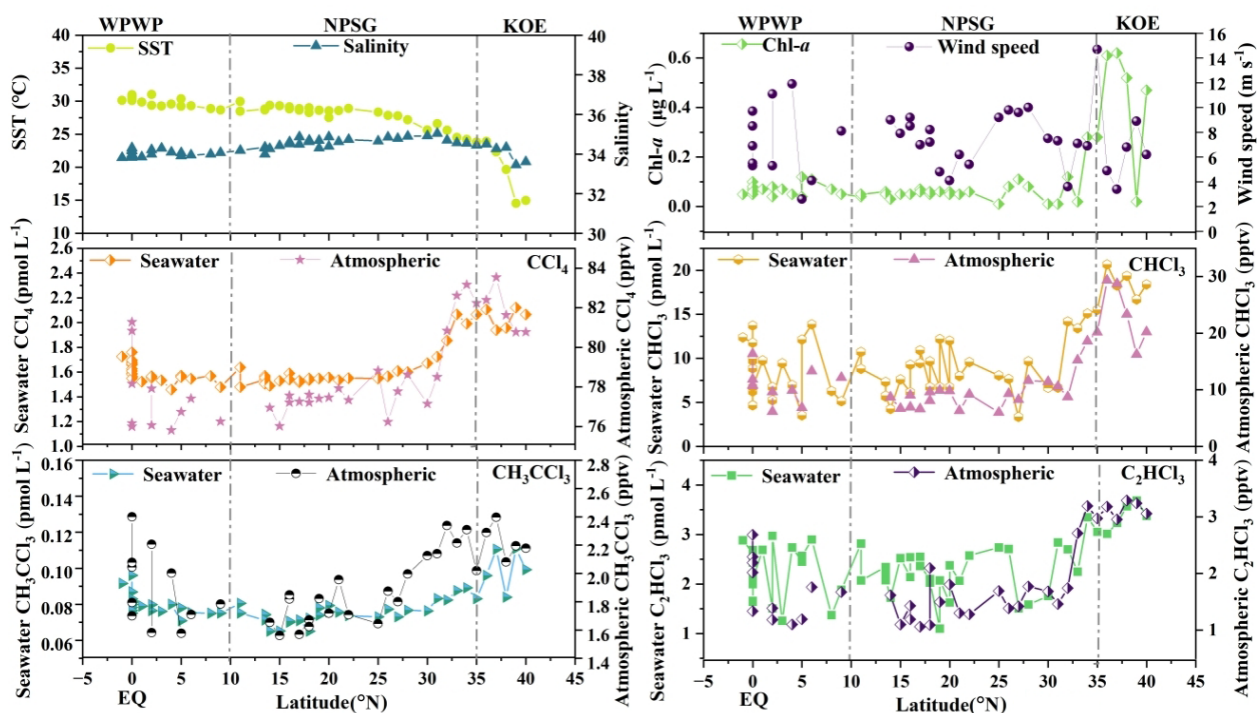
Figure 2. Latitudinal distributions of SST, salinity, and Chl a , and surface seawater and atmospheric concentrations of \text{CCl}_4 , \text{CHCl}_3 , \text{CH}_3\text{CCl}_3 , and \text{C}_2\text{HCl}_3 , along with wind speed in the Western Pacific.
