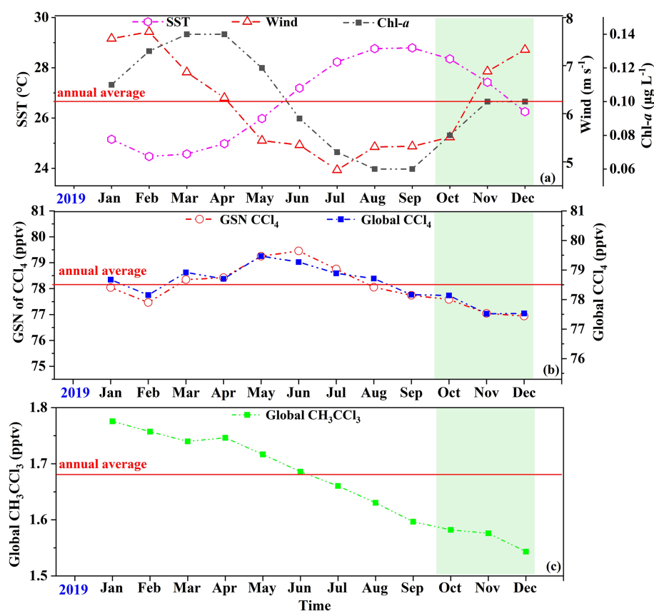
Figure 7. (a) Interannual variations of wind speed, SST, and Chl a concentration in the study area during 2019. (b) Interannual variability of CCl 4 at the GSN site in 2019 compared with the global mean. (c) Interannual variability of CH 3 CCl 3 at the global scale in 2019. Wind speed data were obtained from the ERA5 reanalysis (Hersbach et al., 2020), SST data from the ECCO2 cube92 dataset (Menemenlis et al., 2008), and Chl a data from the NASA Ocean Biology Processing Group (2022). Atmospheric CCl 4 and CH 3 CCl 3 data were obtained from the AGAGE network ( https://agage.mit.edu/ ). Shaded areas indicate the cruise sampling periods.
