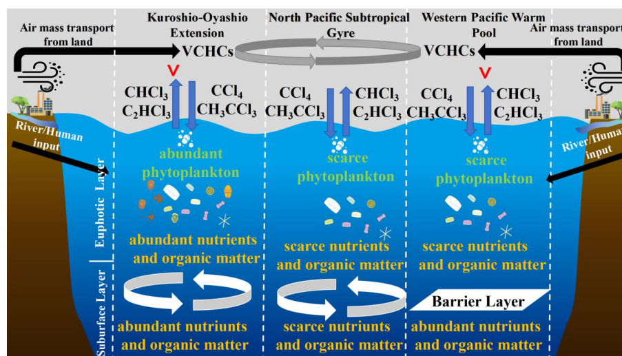
Figure 8. Schematic diagram of key processes and factors controlling the production, distribution, and sea–air interactions of VCHCs in the Western Pacific.
