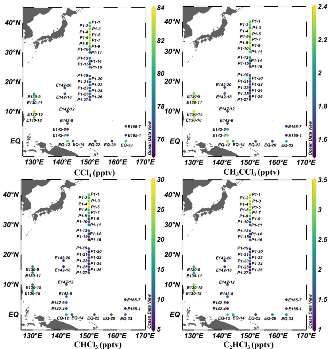
Figure 3. Distributions of \text{CCl}_4 , \text{CH}_3\text{CCl}_3 , \text{CHCl}_3 , and \text{C}_2\text{HCl}_3 in the marine atmospheric boundary layer of the Western Pacific. (Figures generated using Ocean Data View; Schlitzer, Reiner, Ocean Data View, https://odv.awi.de , 2025).
