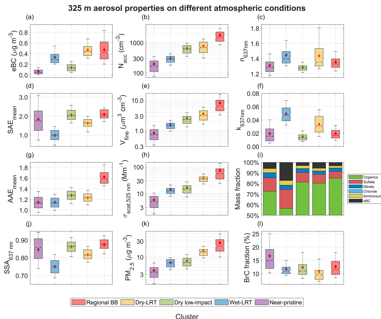
Figure 3. Box plots for the measured variables at the 325 m height when separated by the identified clusters, ordered from 1 to 5. The whiskers extend to the 10th and 90th percentiles, and the mean values are indicated with a red diamond. In (a) the eBC concentration, in (d) the SAE, and in (g) the AAE are the clustering seed variables. In (b) the accumulation mode particles, in (e) the fine mode volume, in (h) the scattering coefficient, and in (k) the \text{PM}_{2.5} mass are the extensive variables. In (c) and (f), the real and imaginary parts of the refractive index, respectively, in (i) the chemical composition, in (j) the SSA, and in (l) the BrC fraction are the other intensive properties. Note that the chemical composition fractions are shown from 50 % to 100 % to facilitate the visualization of more minor differences due to the strong organic aerosol dominance.
