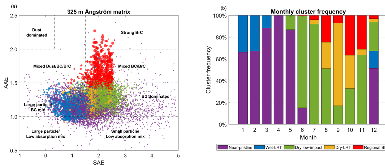
Figure 2. Results for the clustering analysis of the aerosol optical properties at 325 m, using the k -means algorithm with 5 clusters and the binary season separation. In panel (a), the Ångström matrix shows the distribution of clusters, with the point size indicating the equivalent black carbon concentration, and the different highlighted regions relate to possible particle composition as introduced by Cappa et al. (2016). Panel (b) shows the annual cycle of the cluster frequencies.
