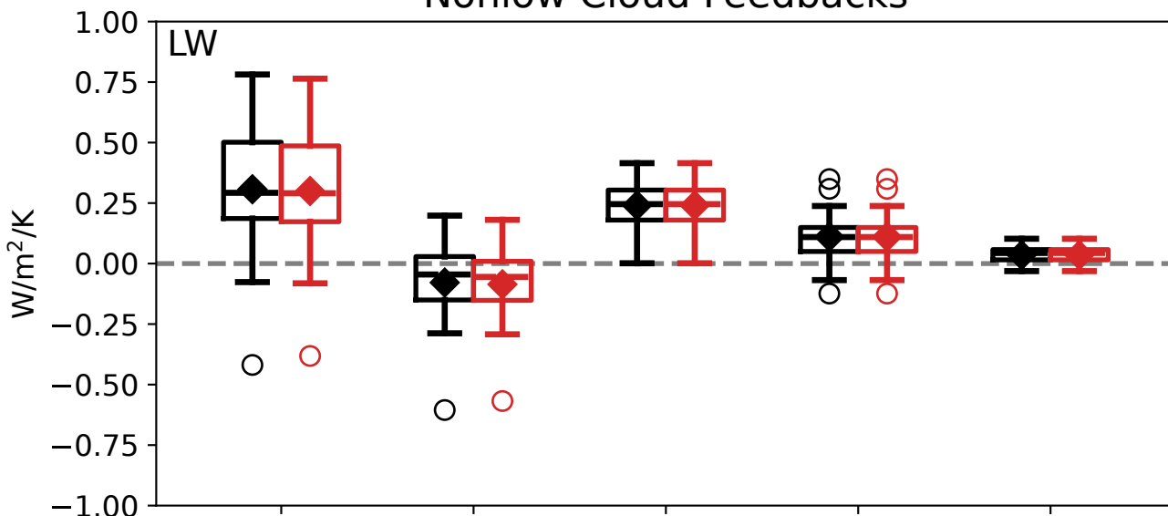
Nonlow Cloud Feedbacks
