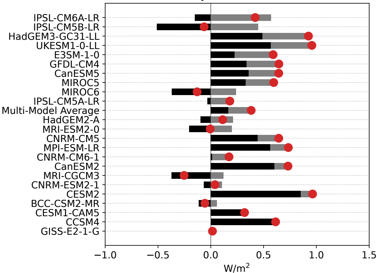
(c) Low Cloud Adjustment
