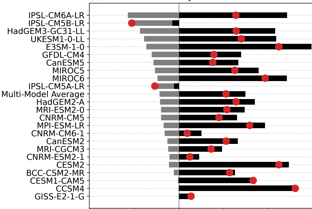
(c) Low Cloud Adjustment
