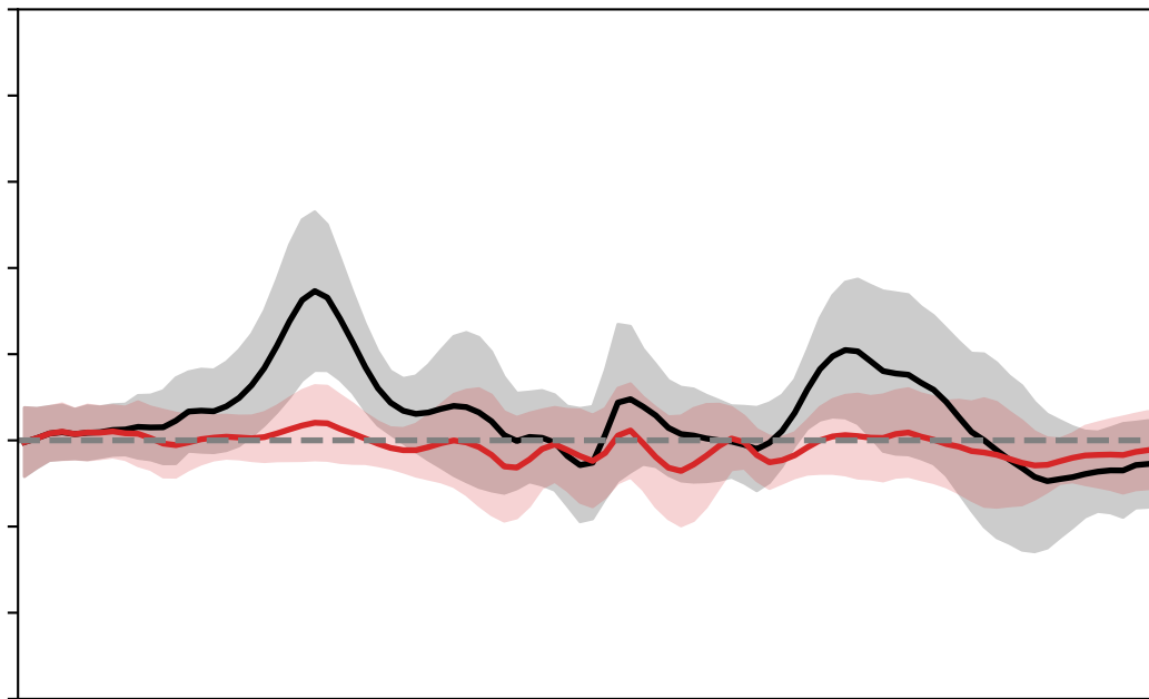
(b) Nonlow Cloud Amount Adjustment
