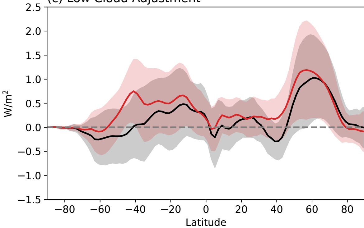
(c) Low Cloud Adjustment
