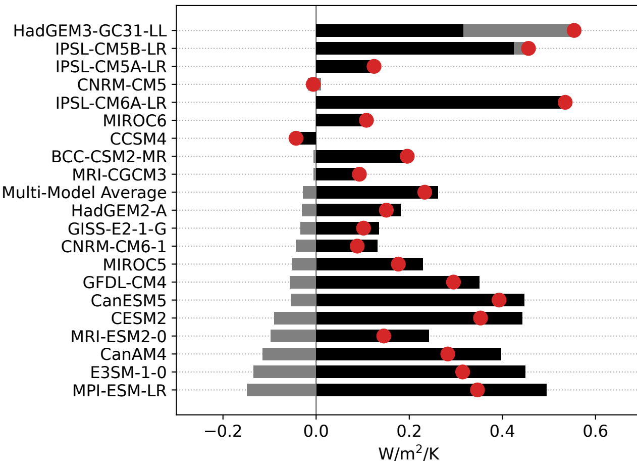
(c) Low Cloud Feedback
