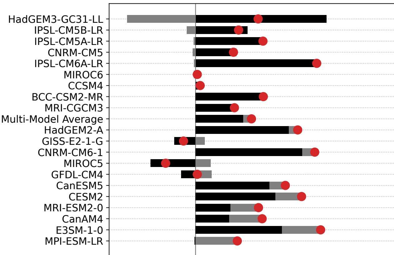
(a) Nonlow Cloud Feedback
