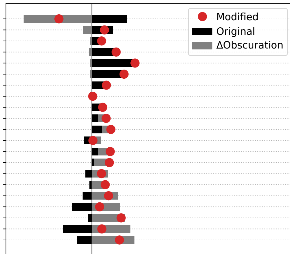
(b) Nonlow Cloud Amount Feedback
