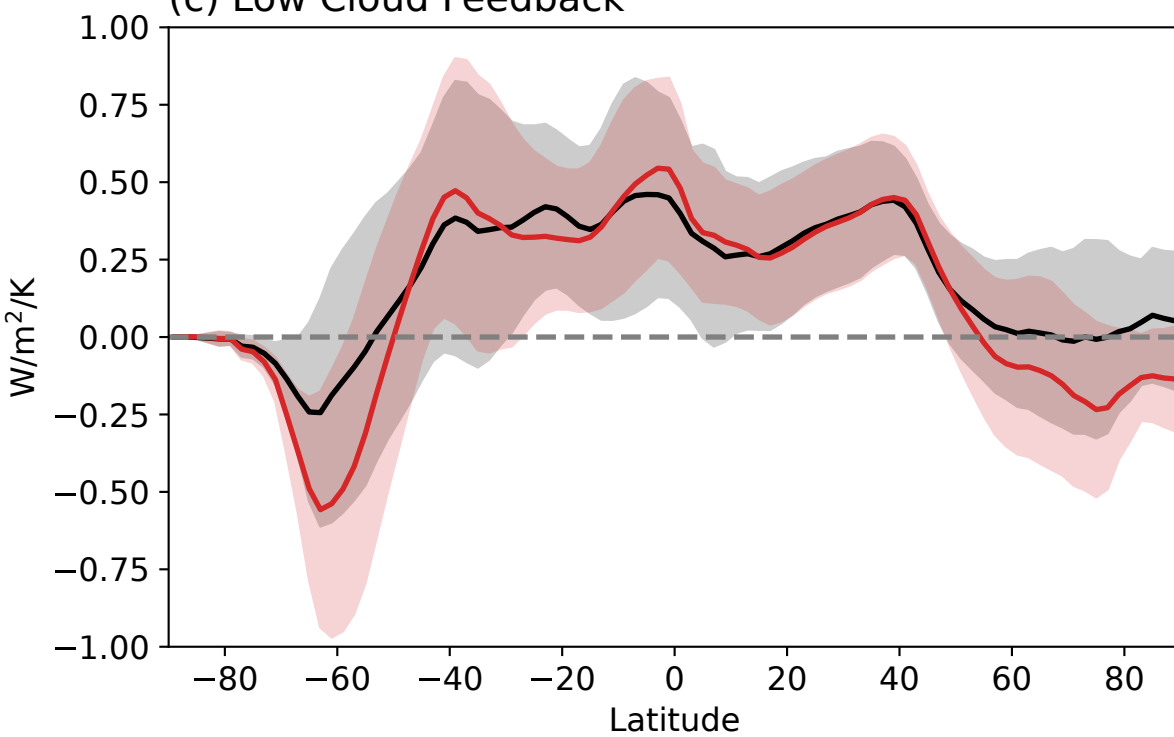
(c) Low Cloud Feedback
