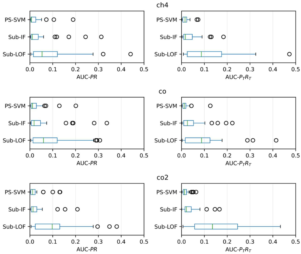
Figure S4: Distribution of the Area Under the Precision-Recall Curve (AUC-PR) score (left column: classic; right column: range-based) for three different outlier detection methods for sequences (for n_s=5 and k=100 ) based on ICOS stations that have at least 30 flags in Level 2 data between April 2021 and March 2024 (for towers the largest available inlet height is used). The green lines indicate the median of the tested stations, the boxes indicate the interquartile range (IQR), while the whiskers extend to up to 1.5 IQR from the edges of the boxes.
