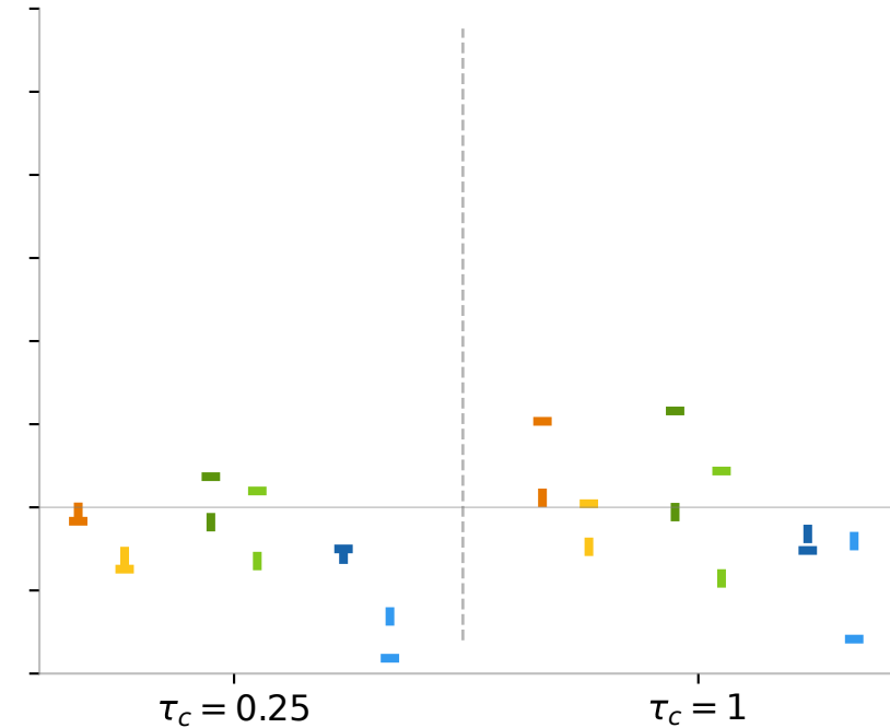
(f) net relative 3D effects
