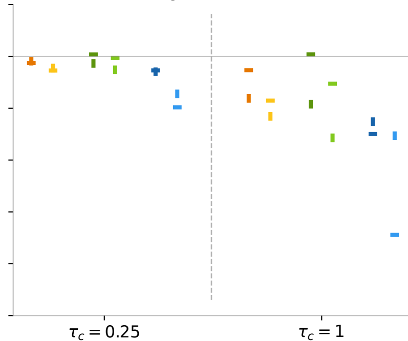
(e) daily relative SW 3D effects
