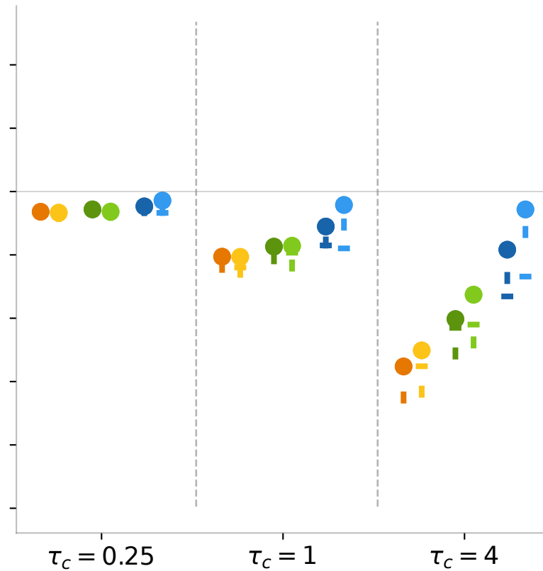
(b) SW oCRE daily
