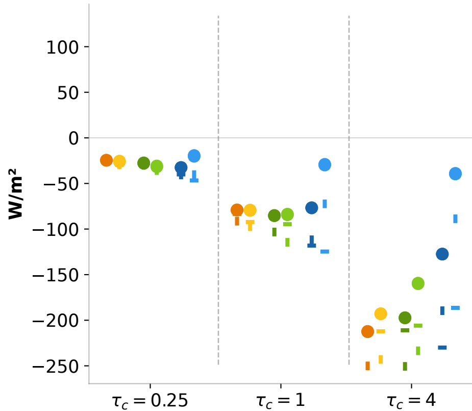
(a) SW oCRE daytime
