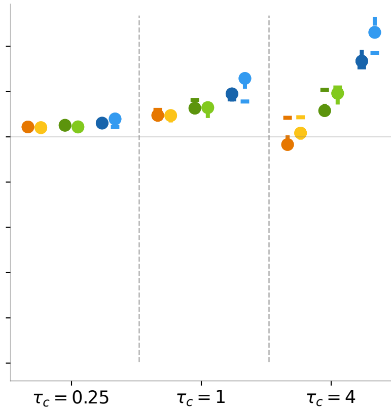
(c) net oCRE
