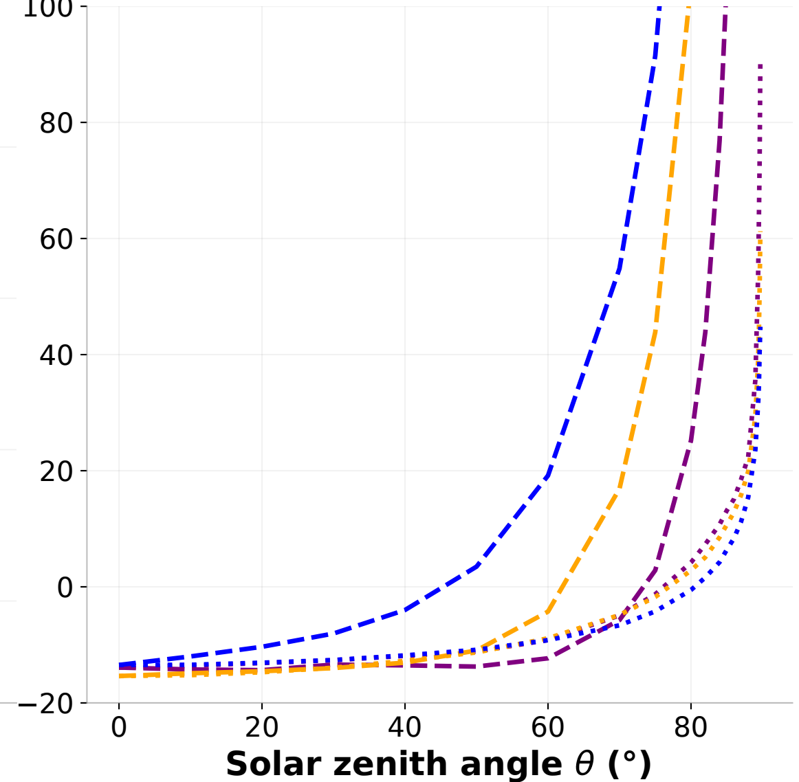
(c) SW 3D effects relative to 1D (%)
