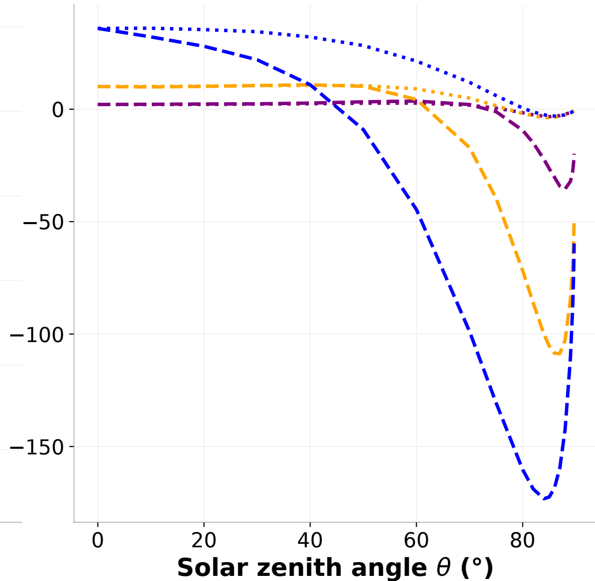
(b) SW 3D effects (W/m 2 )
