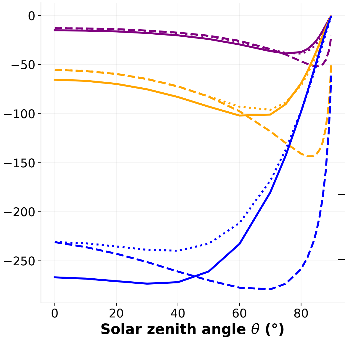
(a) SW oCRE (W/m 2 )
