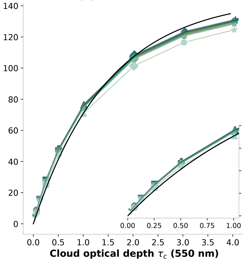
(b) LW overcast CRE
