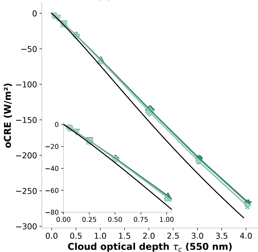
(a) SW overcast CRE
