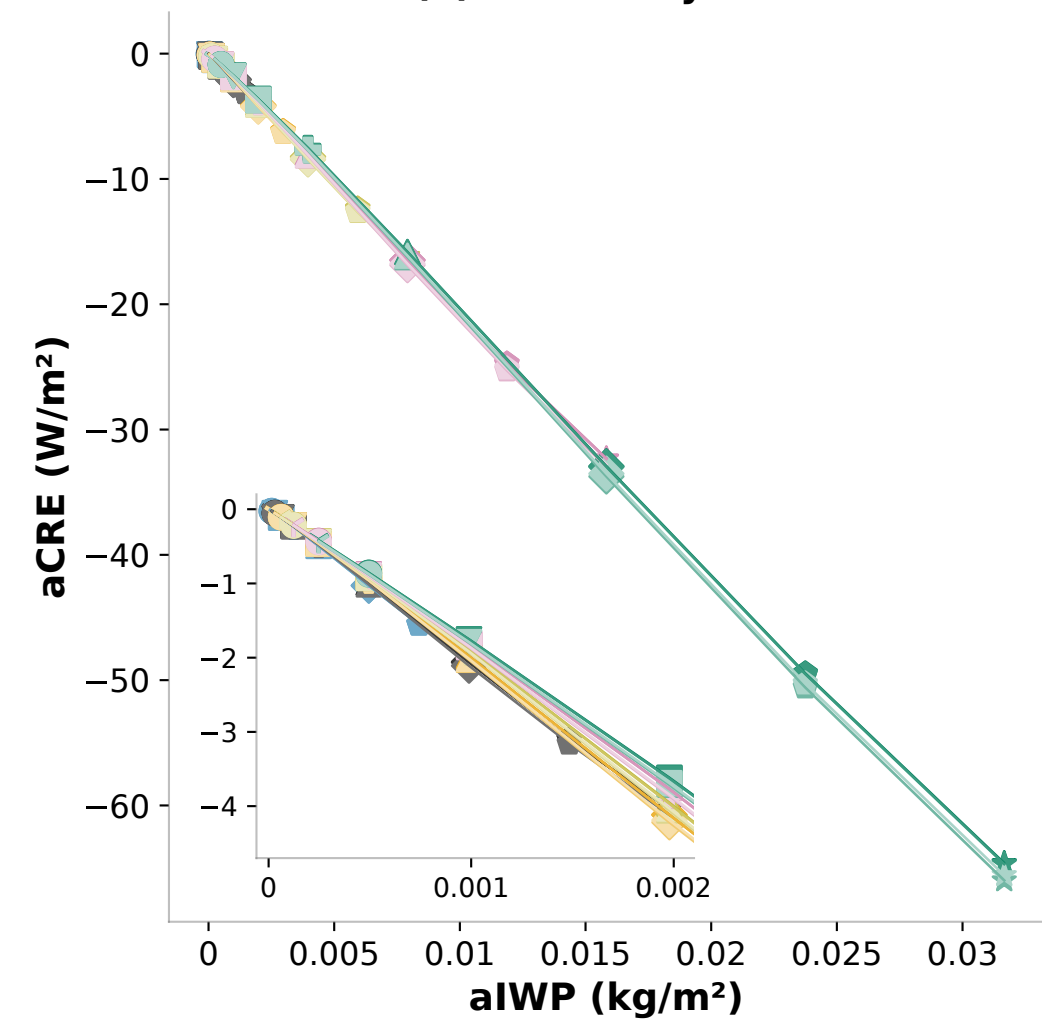
(a) SW all-sky CRE
