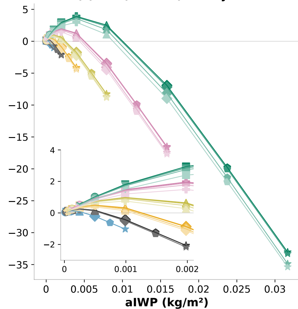
(c) net (LW+SW) all-sky CRE
