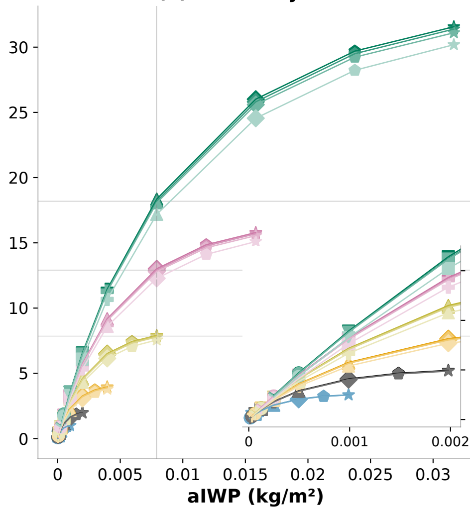
(b) LW all-sky CRE
