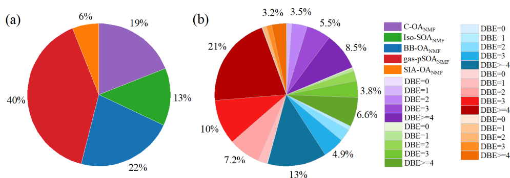
Figure 5. (a) Intensity-based source contributions of each NMF-factor and (b) corresponding classifications based on DBE values. Compounds with DBE values greater than 4 are tentatively considered to possess benzene structures or originate from anthropogenic sources. Relative intensities below 3 % are not labelled.
