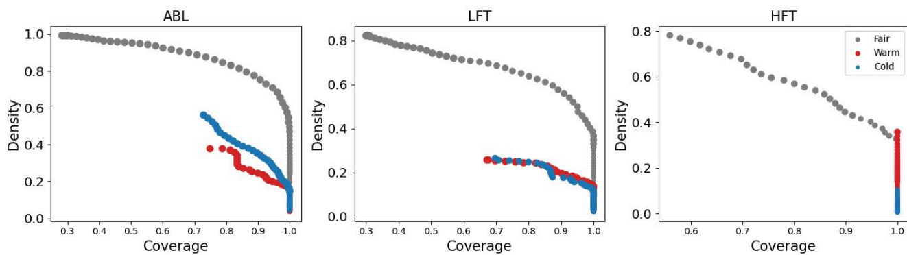
Figure S3: PRIM Coverage-Density-Tradeoff curve (i.e. peeling trajectory) for Winter 2017 ABL (left), LFT (center), and HFT (right) separated by fair weather, warm, and cold airmasses.
