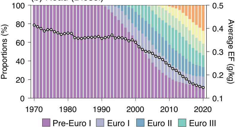
(b) Road (Diesel)
