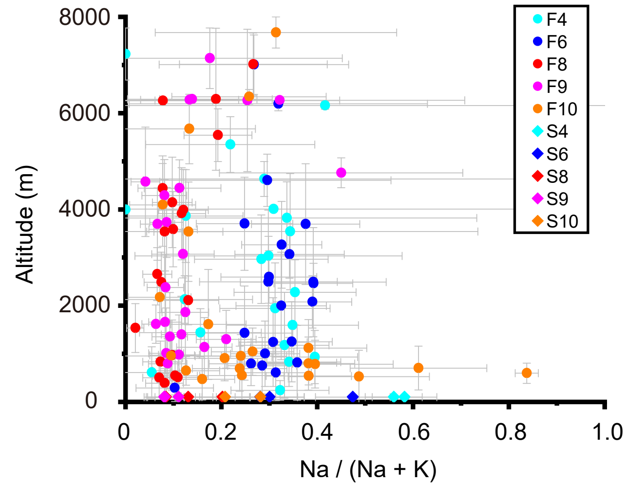
(a) \text{Na} / (\text{Na} + \text{K})
