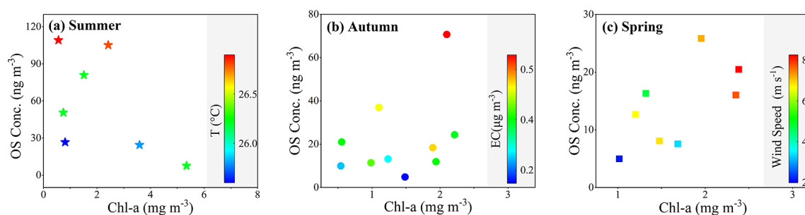
Figure 7. Variations of OSs concentrations as a function of chlorophyll- a (Chl- a ) in (a) summer, (b) autumn, and (c) spring. The markers are colored by air temperature, EC, and wind speed, respectively.
