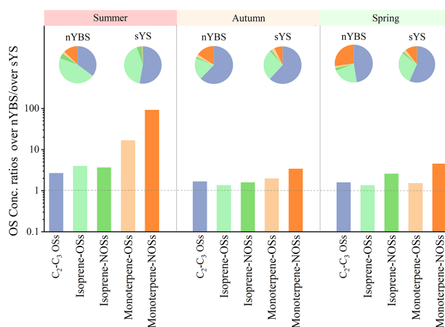
Figure 5. Concentration ratios of atmospheric OSs over the nYBS versus those over the sYS. The pie charts show the relative contribution of OSs compound groups over the nYBS and the sYS during each season.
