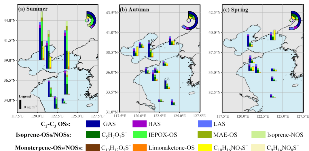
Figure 1. Spatial distributions of OSs in \text{PM}_{2.5} over the YBS during (a) summer, (b) autumn in 2021, and (c) spring in 2022. The inserted charts in panels (a), (b), (c) are the contribution of different OSs compounds. The dotted lines in the panels are the dividing line of the North Yellow Sea (nYS) and the South Yellow Sea (sYS).
