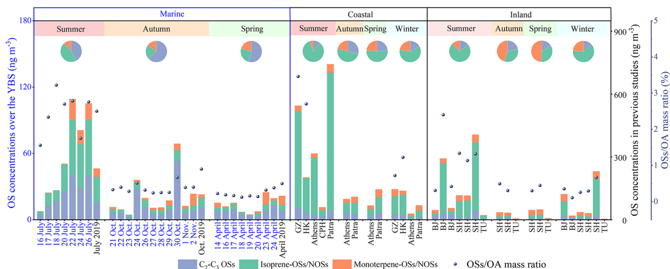
Figure 2. Atmospheric OSs concentrations and mass ratios of (OSs + NOSs) / OA over the YBS in this study and in inland and coastal atmospheres reported in previous studies (Kanellopoulos et al., 2022; Meade et al., 2016; Nguyen et al., 2014; Wang et al., 2020, 2021, 2022b). The data labels in this work are denoted in blue, and those from previous studies are in black. The pie charts represent the average contribution of OSs compound groups in each season. It is noted that the OSs abundance over the YBS and at coastal or inland sites are represented by different y-axes concentration ranges.
