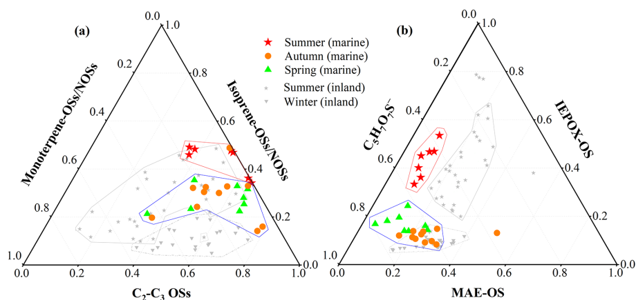
Figure 4. (a) Relative abundance of isoprene OSs, monoterpene OSs, and C_2 – C_3 OSs, and (b) composition of isoprene OSs over the YBS in summer (red), autumn (orange) and spring (green). The results previously reported at the inland urban site (Wang et al., 2020) are colored gray.
