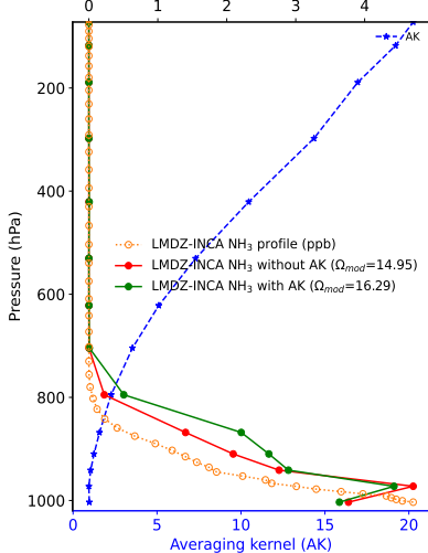
(a) location: (25.578, 87.655), Date: 2019-02-24 NH 3 profile (ppb) NH 3 sub-columns ( 10^{15} molec. cm -2 )
