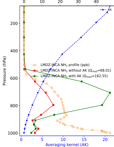
(b) location: (25.509, 87.682), Date: 2019-03-30 NH 3 profile (ppb) NH 3 sub-columns ( 10^{15} molec. cm -2 )
