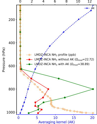
(c) location: (25.587, 87.538), Date: 2019-10-28 NH 3 profile (ppb) NH 3 sub-columns ( 10^{15} molec. cm -2 )
