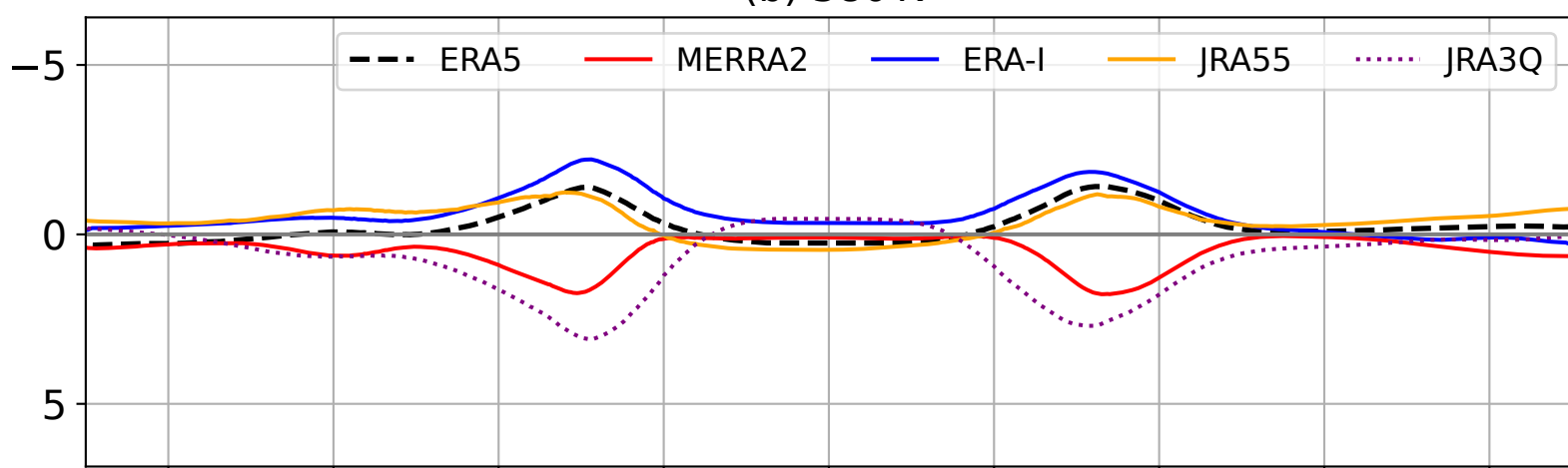
(c) PPT10mean
