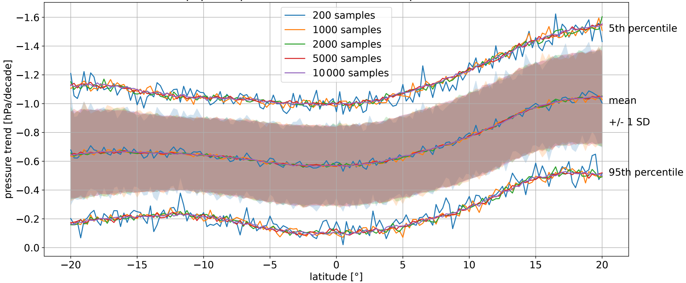
DLM sample experiment (tropopause pressure DLM trends at cold point 1998-2019)
