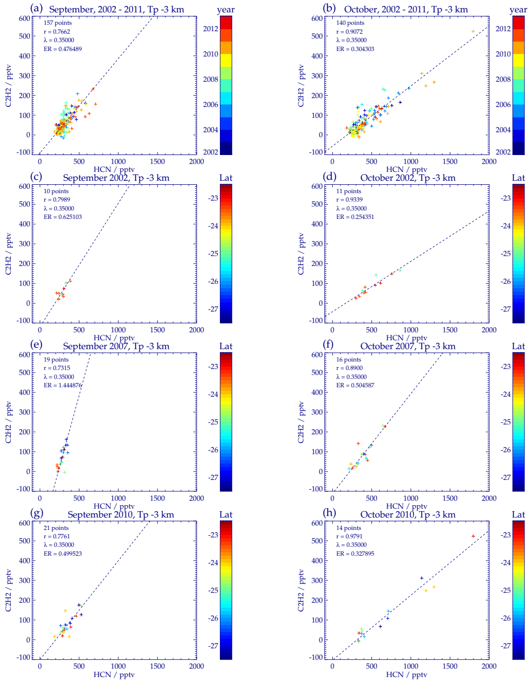
Figure S9. Top row: Correlation plots between (a) September and (b) October composites (right) of MIPAS C 2 H 2 and HCN at 3 km below the tropopause for measurements in a bin between Mozambique and southern Madagascar (27.5°S-22.5°S, 30°E-45°E, see Fig. 10 of the main manuscript). Given in the legend are the number of data pairs, the Pearson correlation coefficient r , the applied \lambda value and the fitted enhancement ratio ER. Second, third and bottom row: Same as upper row, but for September/October (c, d) 2002, (e, f) 2007 and (g, h) 2010.
