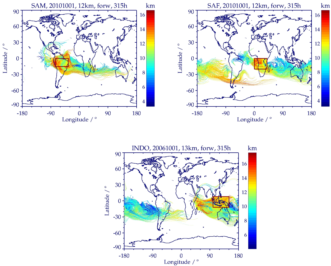
Figure S8. HYSPLIT 13-day forward trajectories started on October 1, 2010, at 12 km altitude above the South American (top left) and the South African (top right) biomass burning region. Bottom: 13-day forward trajectories started on October 1, 2006, at 13 km altitude above the Indonesian biomass burning region.
