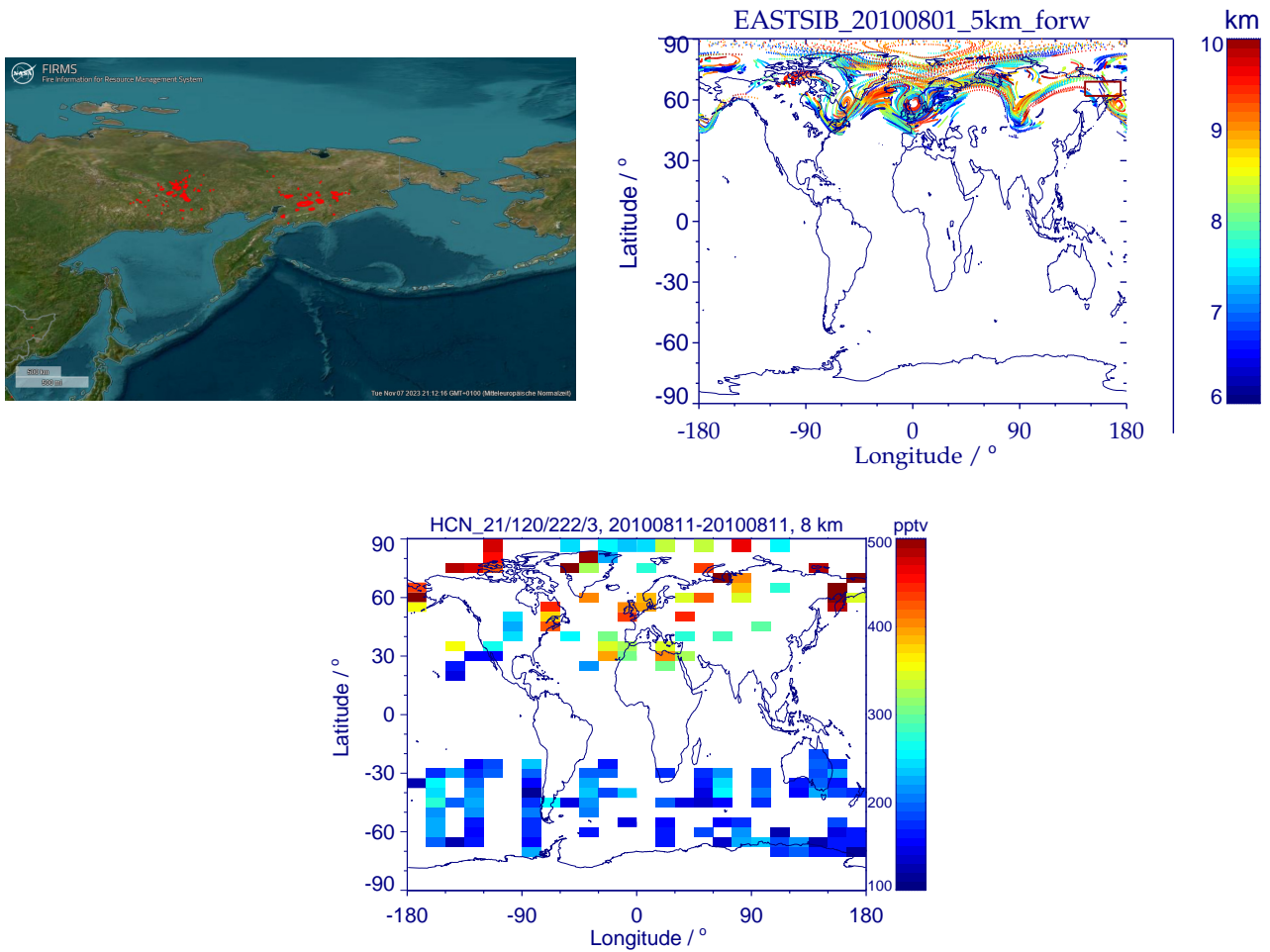
Figure S6. Top left: MODIS fire counts from 1 August 2010 in North-East Siberia, plotted with the graphical interface on the FIRMS-website. Top right: HYSPLIT 11-day forward trajectories started on August 1, 2010, 0:00 UT, at 5 km altitude above the fire region (marked by red margin), color-coded by altitude. Only the sections of the trajectories covering the 11th of August are shown. Bottom: MIPAS HCN distribution at 8 km altitude, measured on August 11, 2010.
