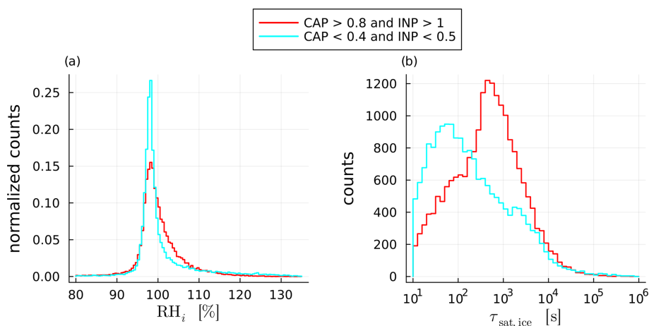
Figure 13. Histograms for (a) RH_i and (b) \tau_{\text{sat,ice}} at the end of the ascent for only the fast ascending trajectories and PPE members with both CAP > 0.8 and INP scaling factor > 1 (red) or CAP < 0.4 and INP scaling factor < 0.5 (cyan).
