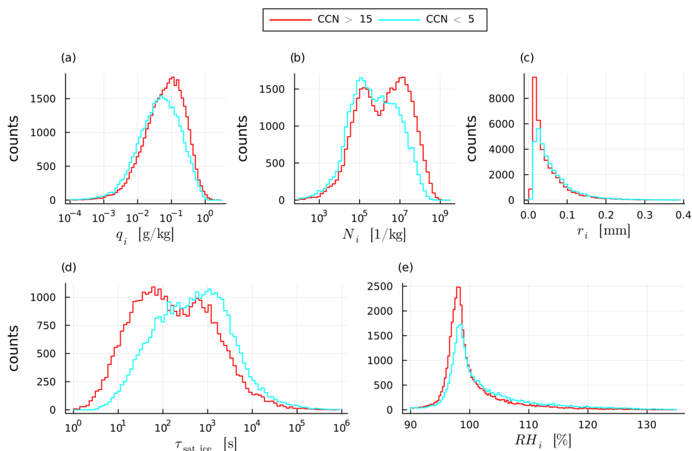
Figure 15. Histograms for q_i in (a), N_i in (b), r_i in (c), \tau_{\text{sat,ice}} in (d) and RH_i in (e) at the end of the ascent for only the fast ascending trajectories and PPE members with a CCN scaling factor larger than 15 (red; 17 PPE members and 686 947 trajectories) or smaller than 5 (cyan; 17 PPE members and 627 912 trajectories).
