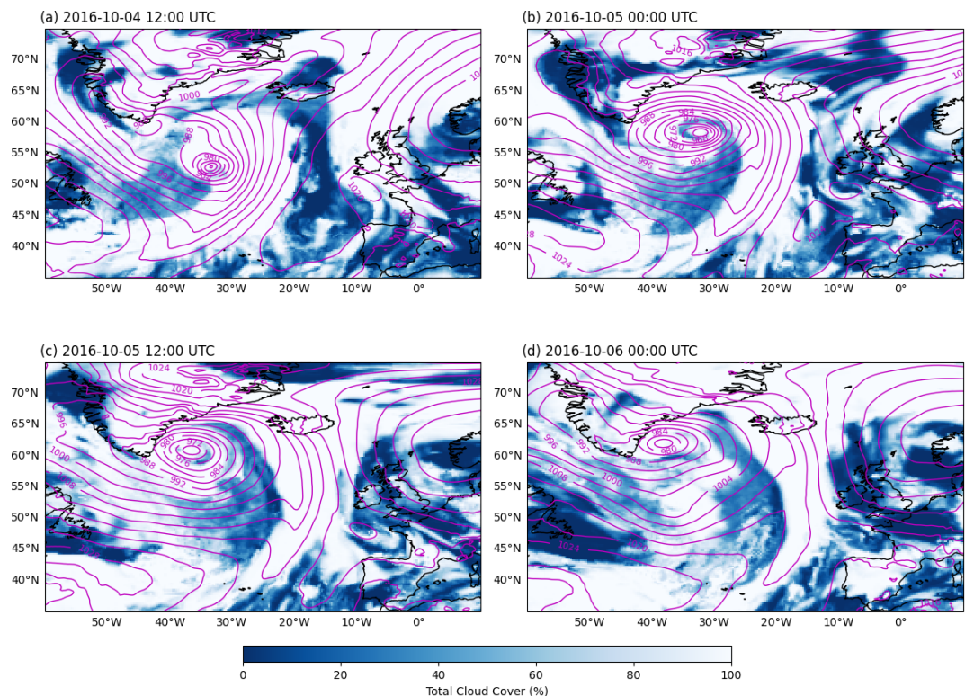
Figure 1. ERA5 data showing the total cloud cover and sea level pressure at 4 October 2016 12:00 UTC in (a), 5 October 2016 00:00 UTC in (b), 5 October 2016 12:00 UTC in (c) and 6 October 2016 00:00 UTC in (d).
