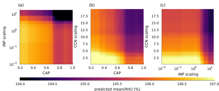
Figure 7. Two dimensional PDPs for RF^2_{\text{mean}(RH_i)} for INP vs. CAP in (a), CCN vs. CAP in (b) and CCN vs. INP in (c).
