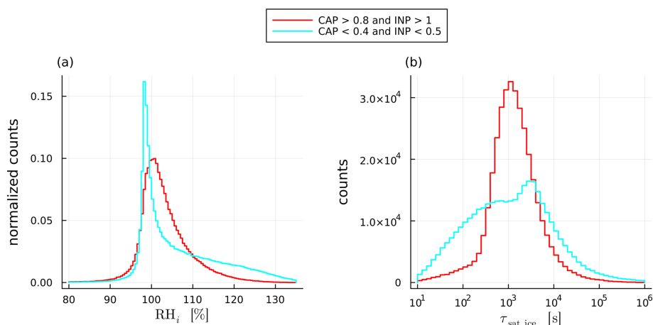
Figure 9. Histograms for (a) RH_i and (b) \tau_{\text{sat,ice}} at the end of the ascent for all PPE members with CAP > 0.8 and INP scaling factor > 1 (red; in total 9 PPE members and 357 888 trajectories) or CAP < 0.4 and INP scaling factor < 0.5 (cyan; in total 9 PPE members and 363 512 trajectories).
