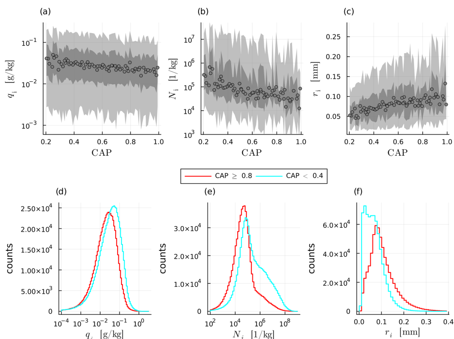
Figure 4. (a) q_i , (b) N_i and (c) ice radius ( r_i ) at the end of the ascent over CAP, with makers showing median values and shaded areas the 5th to 95th percentiles (light grey) and 25th to 75th percentiles (dark grey). Panels (d), (e), and (f) show q_i , N_i and r_i at the end of the ascent respectively, but as histograms for all PPE members with CAP values either larger than 0.8 (red; in total 16 PPE members and 633 400 trajectories) or smaller than 0.4 (cyan; in total 18 PPE members and 696 846 trajectories).
