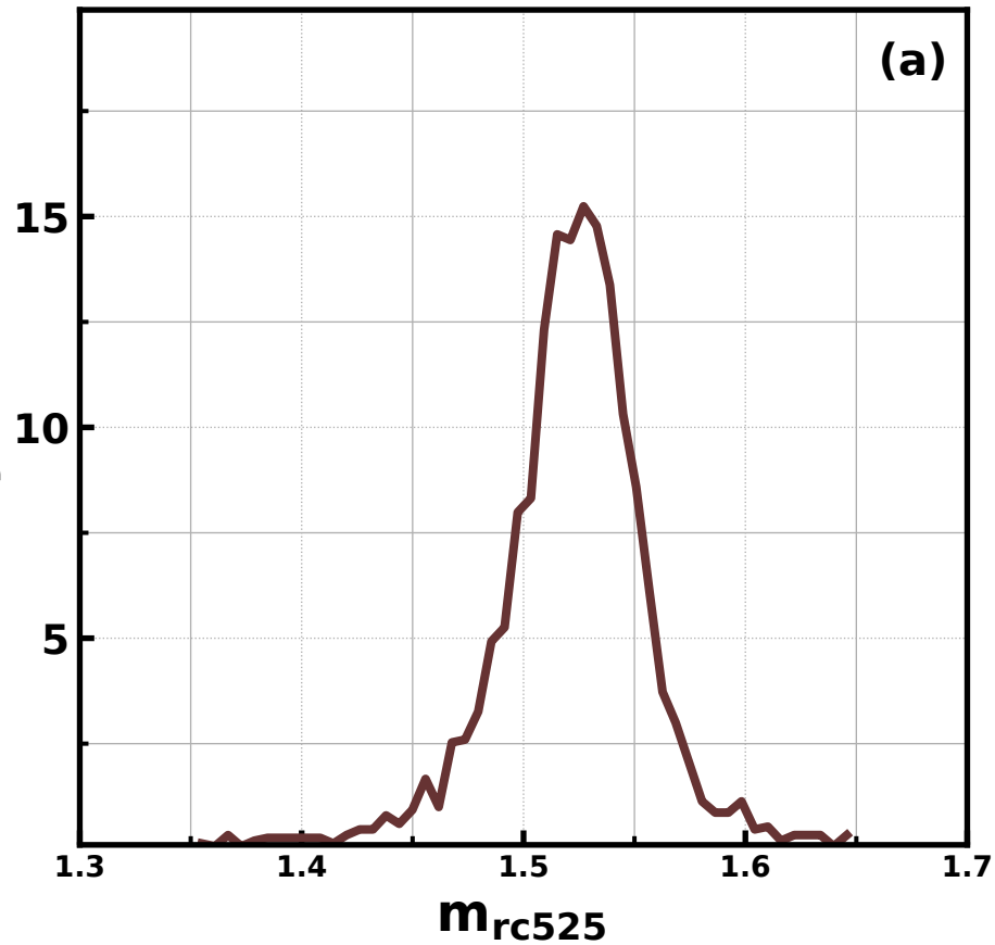
Probability Distribution
