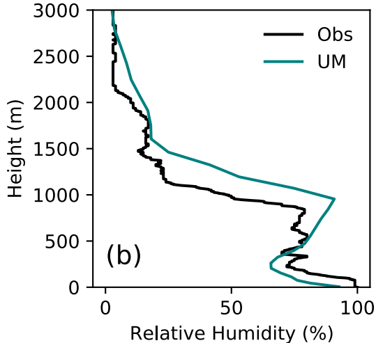
LANFEX: Nov 24 22:00 UTC
