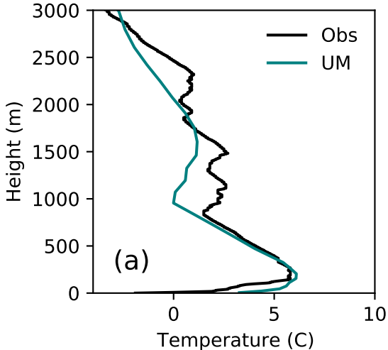
LANFEX: Nov 24 22:00 UTC
