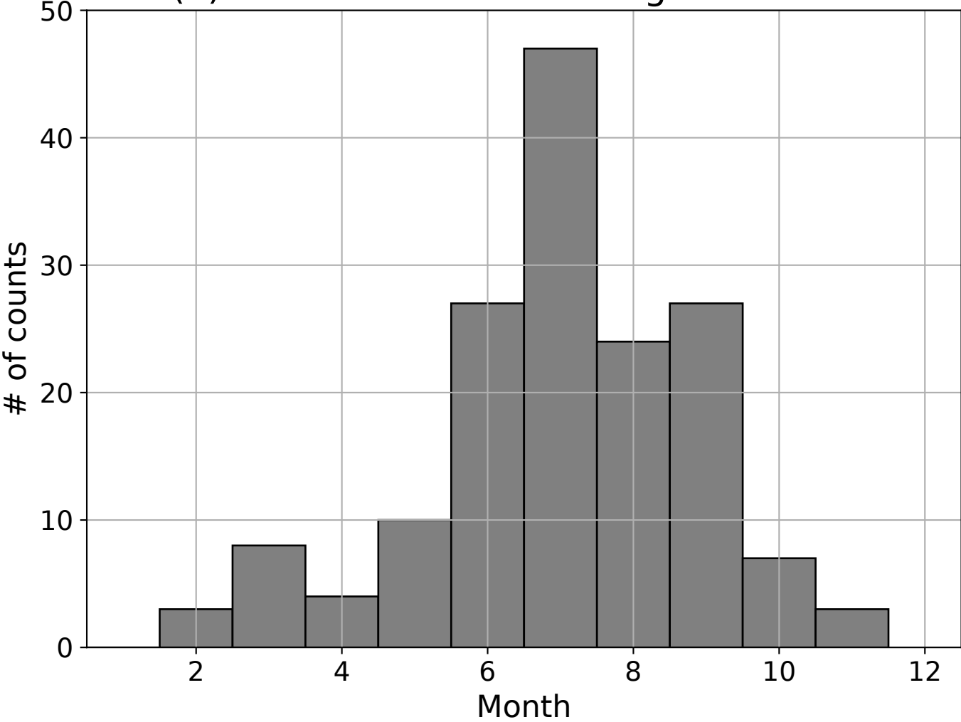
(a) Convective clouds histogram: Month
