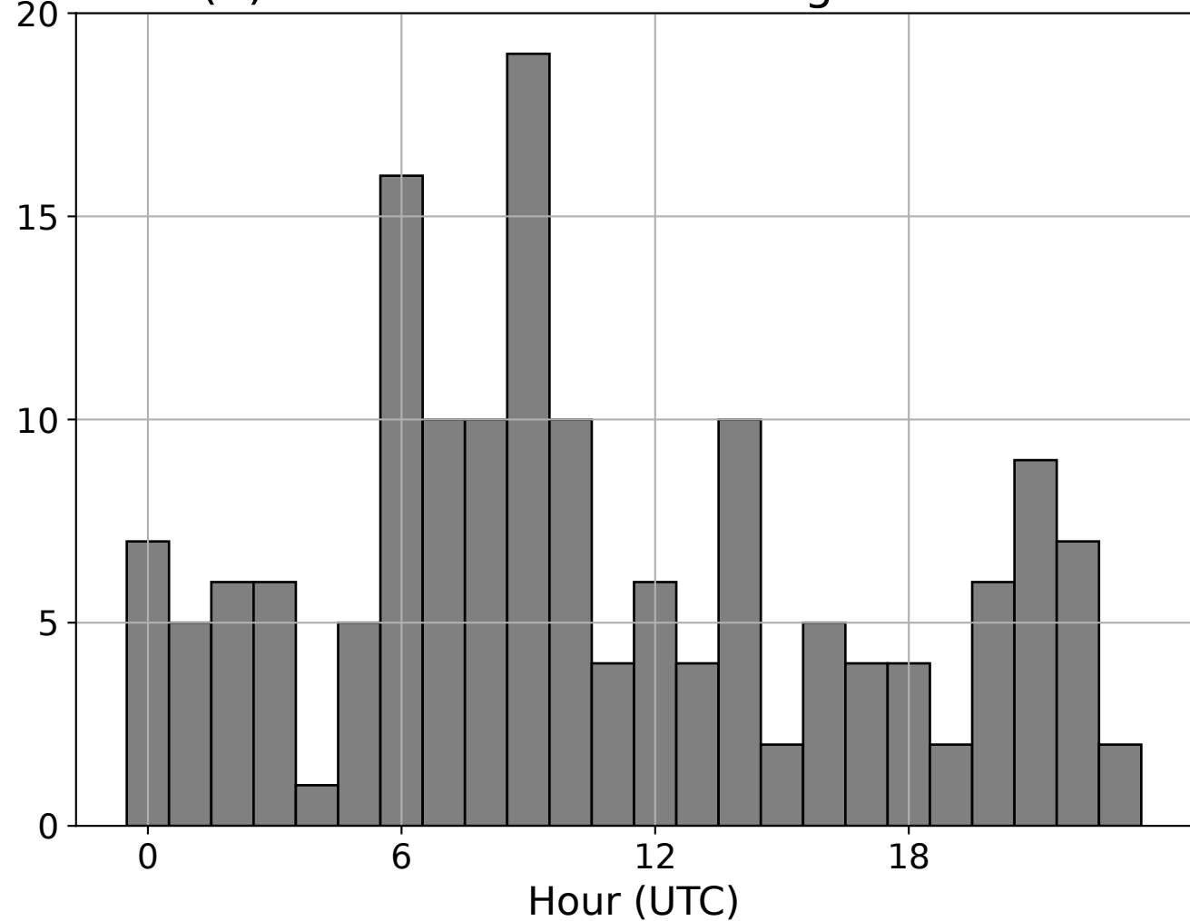
(b) Convective clouds histogram: Hour
