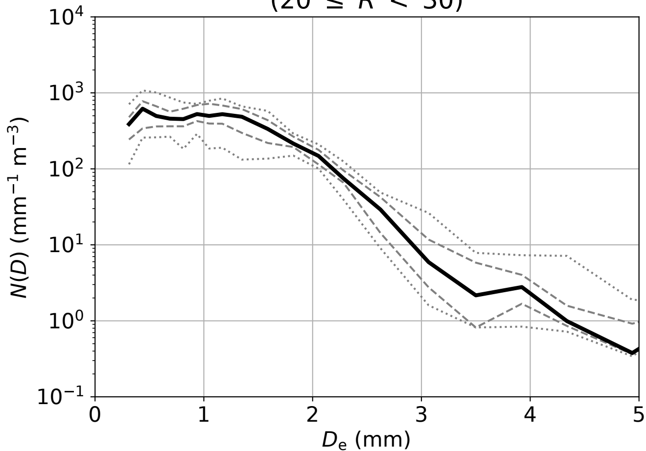
(c) DSD at Kumagaya: # of DSDs = 21 ( 20 \leq R < 30 )
