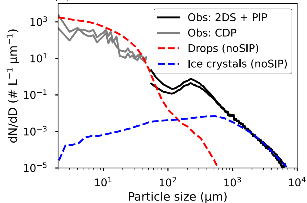
(a) noSIP: 5 to 6 km
