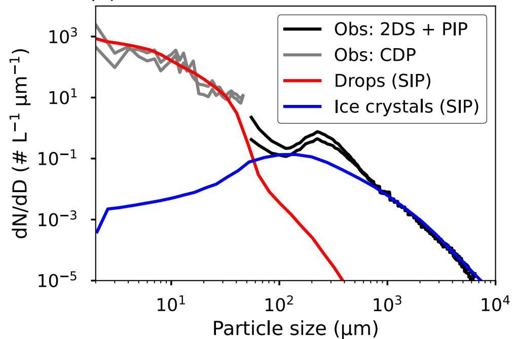
(b) SIP: 5 to 6 km
