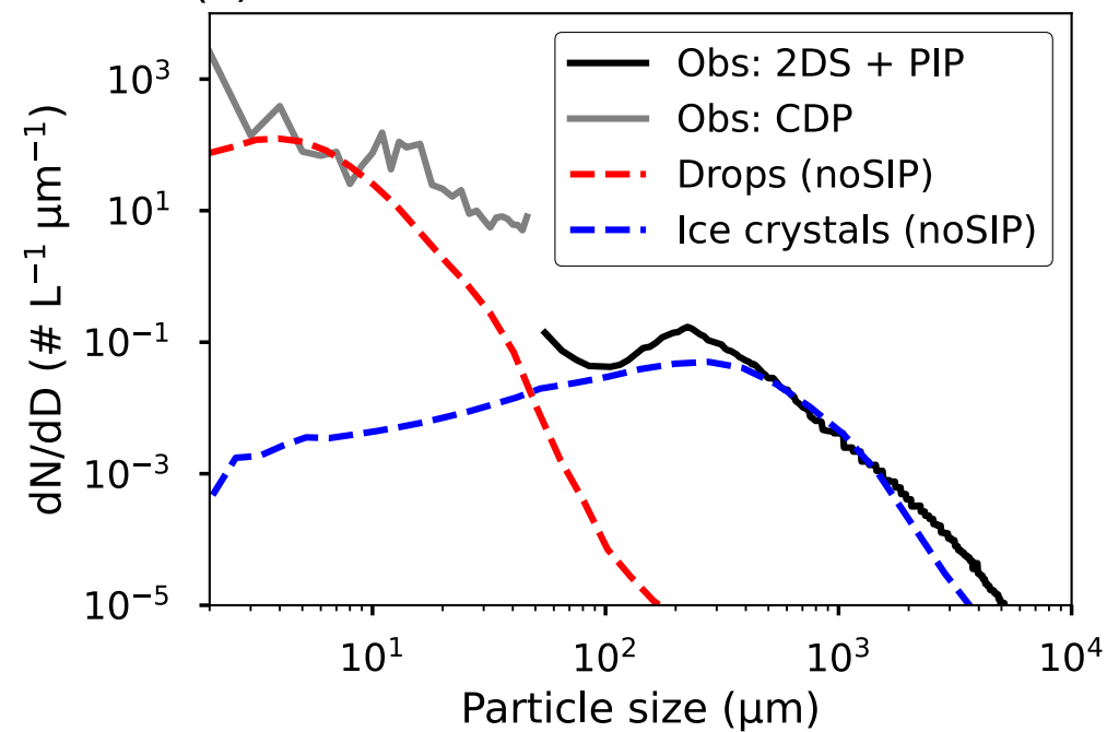
(c) noSIP: 7 to 7.5 km
