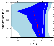
(g) Relative humidity wrt Ice
