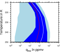
(a) DEP Ice content
