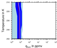
(b) HOM Ice content
