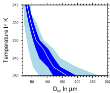
(f) Total cloud Ice size
