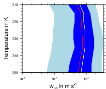
(h) Upward vertical velocity
