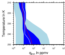
(c) IMM Ice content
