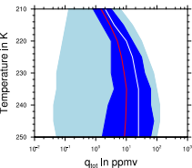
(e) Total cloud Ice content
