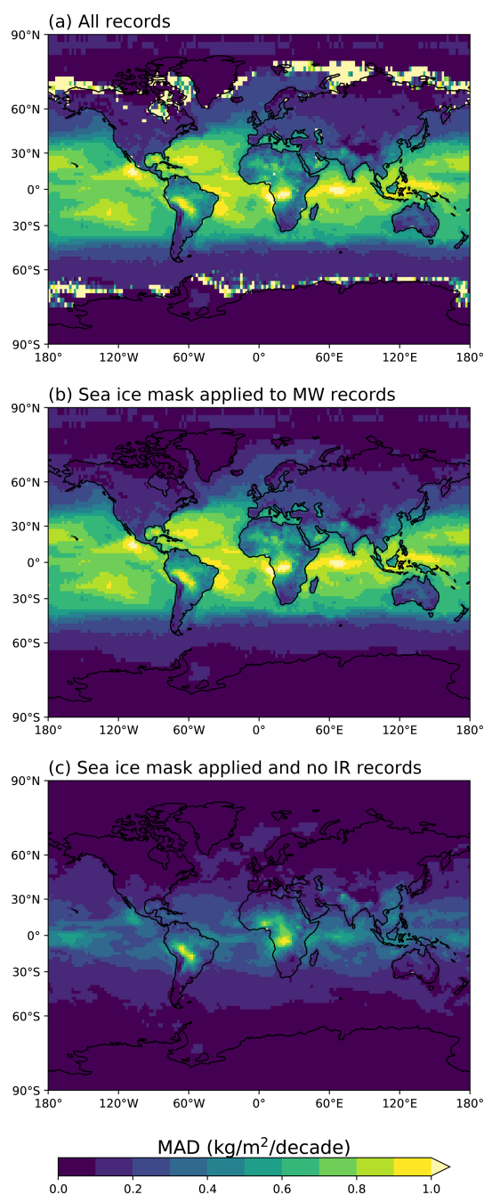
Figure 9. Mean absolute deviation (MAD) of archive total column water vapour (TCWV) trend estimates for the period between 1988–2014 (a). High MAD values observed in the tropics are on the order of 25 % of observed trends, while the highest MAD values ( > 1.0 \text{ kg m}^{-2} per decade) are observed at high latitudes and are related to sea ice. Application of the sea-ice mask (see Fig. 2) to the microwave (MW) records removes these effects seen at high latitudes (b), while the high variability seen in the tropics is related to the infrared-only products (c).
