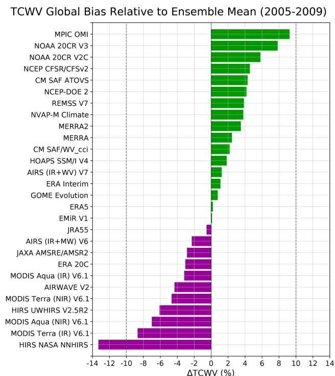
Figure 6. Global TCWV differences of each archive member to the ensemble mean ( \Delta TCWV) for the common period (2005–2009), with the dashed line indicating \pm 2\sigma . Average global differences have been summed and then normalised by the ensemble mean TCWV. For records that have missing data over land or polar regions, the ensemble mean is recalculated to account for differences, excluding these areas with missing data.
