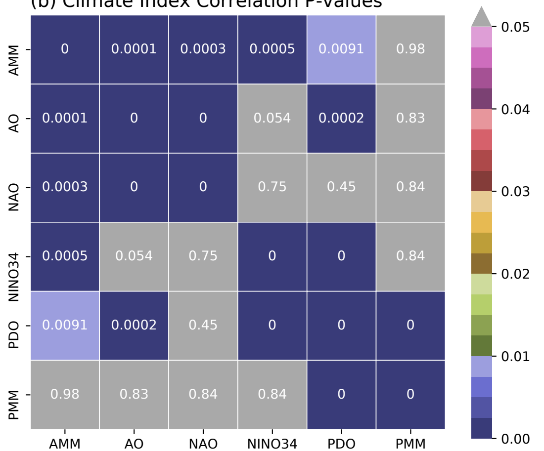
(b) Climate Index Correlation P-values
