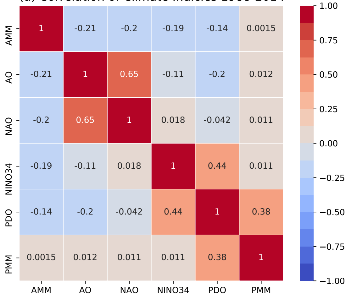
(a) Correlation of Climate Indices 1988-2014
